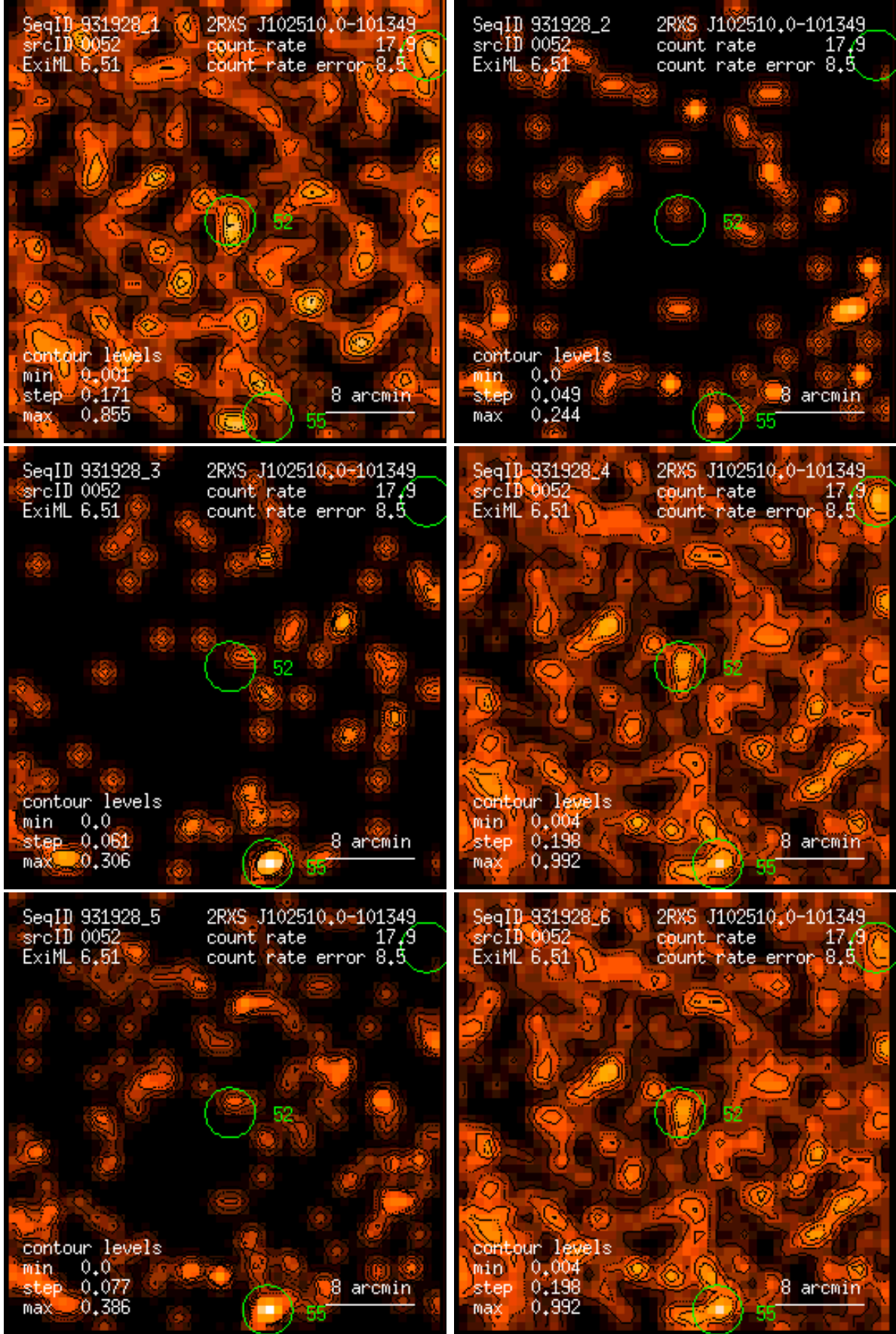
Figure 52: RASS 931928: detection 0052: band rate images, Gaussian filter: (1) PSPC channels 11 – 41, (2) 52 – 90, (3) 91 – 201, (4) 11 – 235, (5) 52 – 201, (6) 11 – 201. Broad band rates in counts/ks. Band rate contour levels in counts/ks/arcmin 2 .
