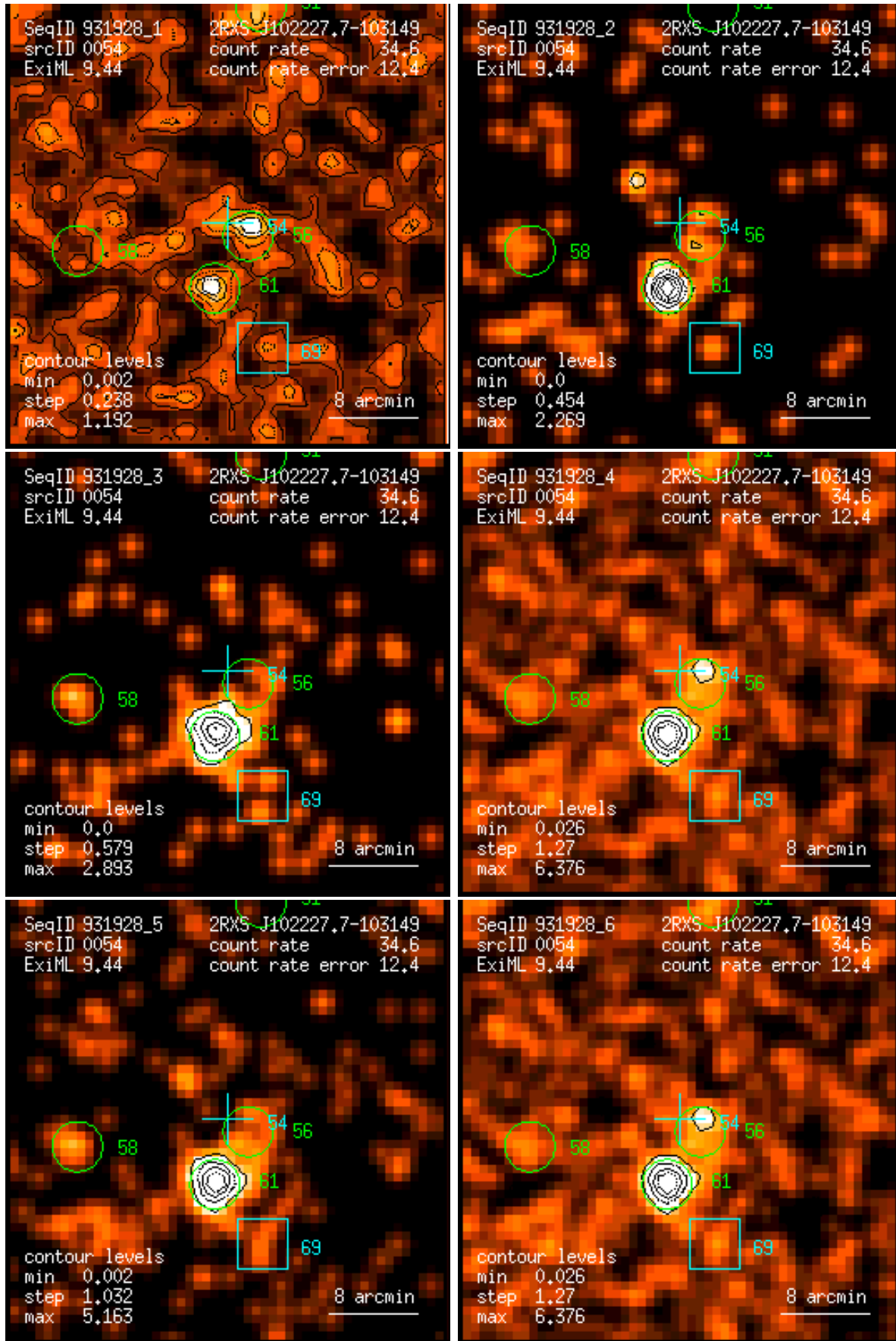
Figure 54: RASS 931928: detection 0054: band rate images, Gaussian filter: (1) PSPC channels 11 – 41, (2) 52 – 90, (3) 91 – 201, (4) 11 – 235, (5) 52 – 201, (6) 11 – 201. Broad band rates in counts/ks. Band rate contour levels in counts/ks/arcmin 2 .
