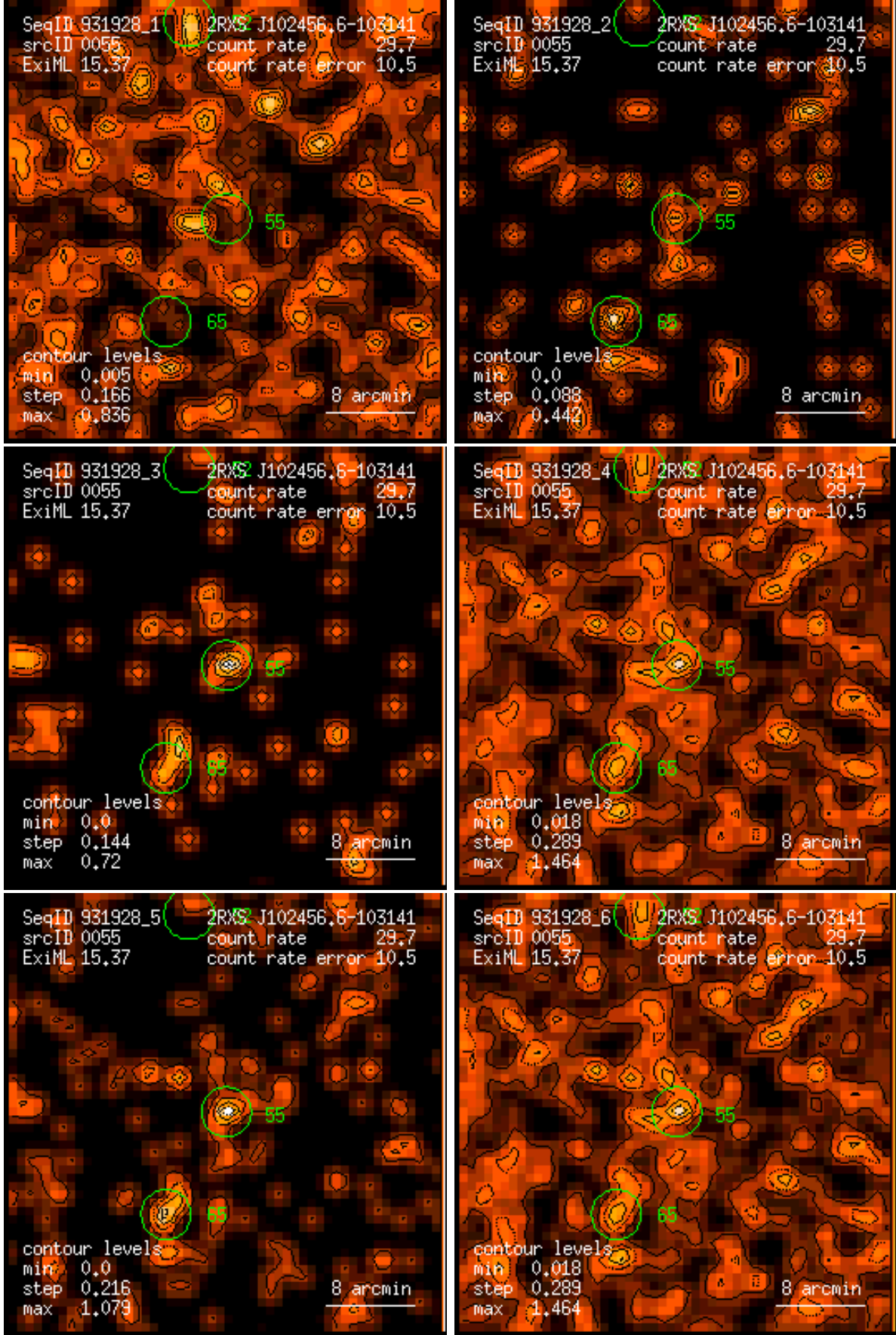
Figure 55: RASS 931928: detection 0055: band rate images, Gaussian filter: (1) PSPC channels 11 – 41, (2) 52 – 90, (3) 91 – 201, (4) 11 – 235, (5) 52 – 201, (6) 11 – 201. Broad band rates in counts/ks. Band rate contour levels in counts/ks/arcmin 2 .
