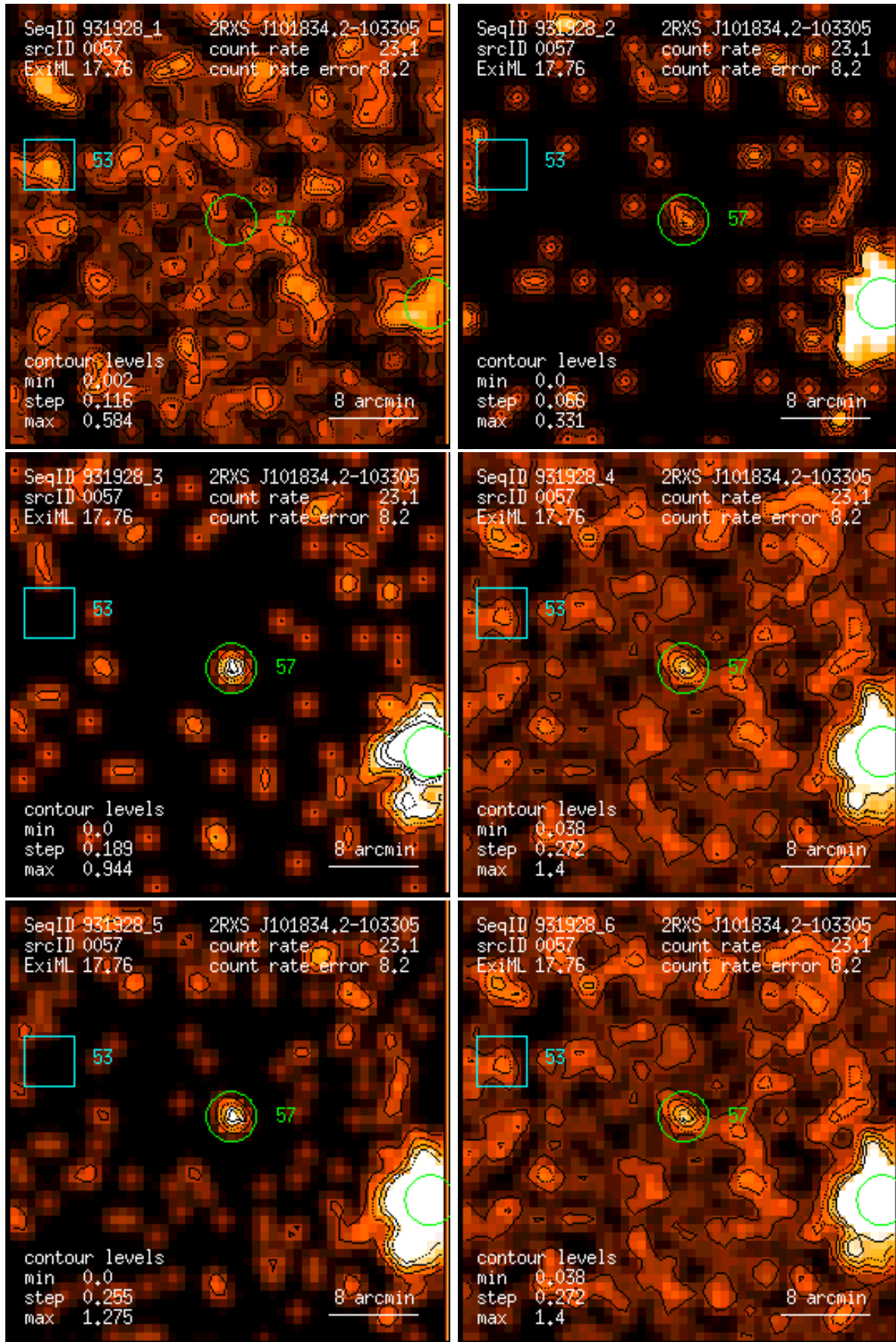
Figure 57: RASS 931928: detection 0057: band rate images, Gaussian filter: (1) PSPC channels 11 – 41, (2) 52 – 90, (3) 91 – 201, (4) 11 – 235, (5) 52 – 201, (6) 11 – 201. Broad band rates in counts/ks. Band rate contour levels in counts/ks/arcmin 2 .
