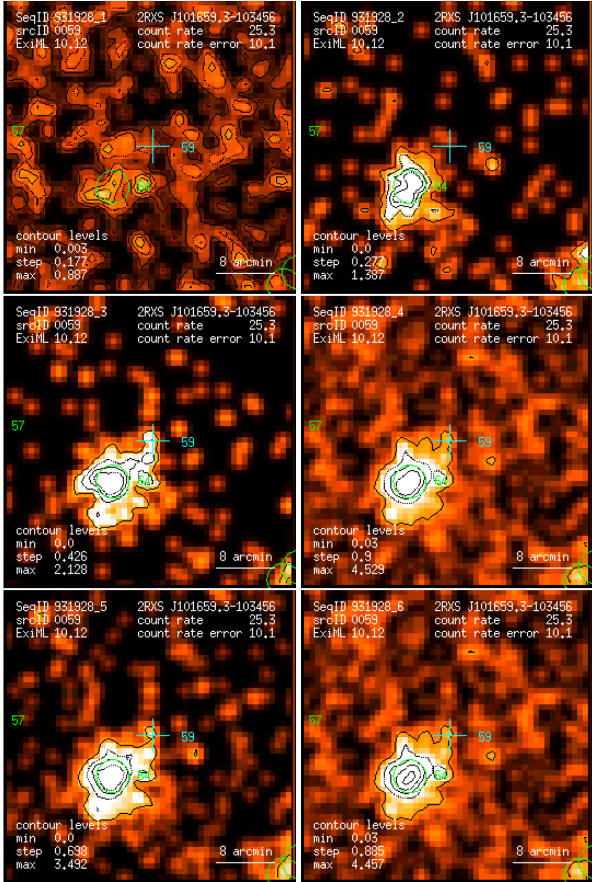
Figure 59: RASS 931928: detection 0059: band rate images, Gaussian filter: (1) PSPC channels 11 – 41, (2) 52 – 90, (3) 91 – 201, (4) 11 – 235, (5) 52 – 201, (6) 11 – 201. Broad band rates in counts/ks. Band rate contour levels in counts/ks/arcmin 2 .
