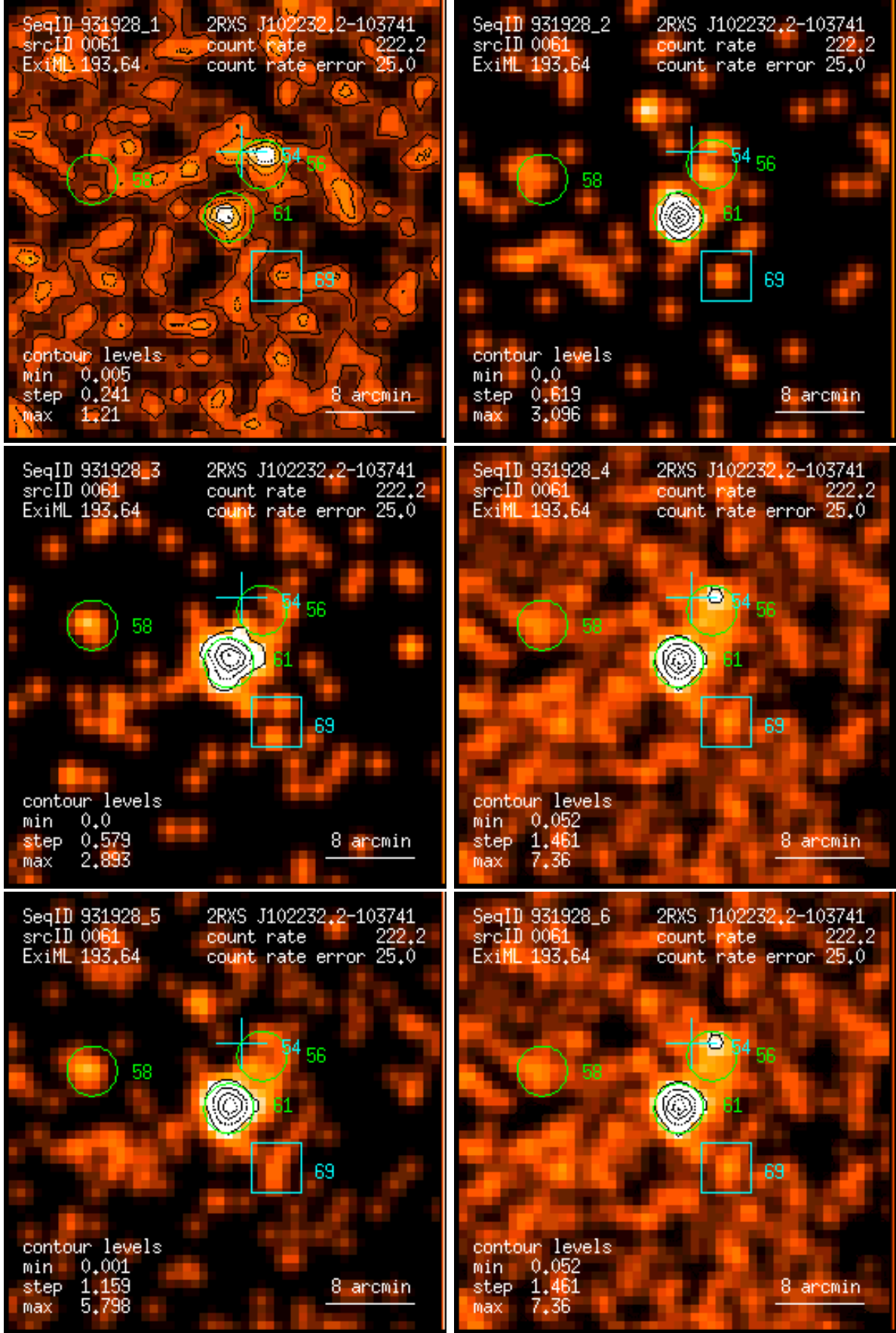
Figure 61: RASS 931928: detection 0061: band rate images, Gaussian filter: (1) PSPC channels 11 – 41, (2) 52 – 90, (3) 91 – 201, (4) 11 – 235, (5) 52 – 201, (6) 11 – 201. Broad band rates in counts/ks. Band rate contour levels in counts/ks/arcmin 2 .
