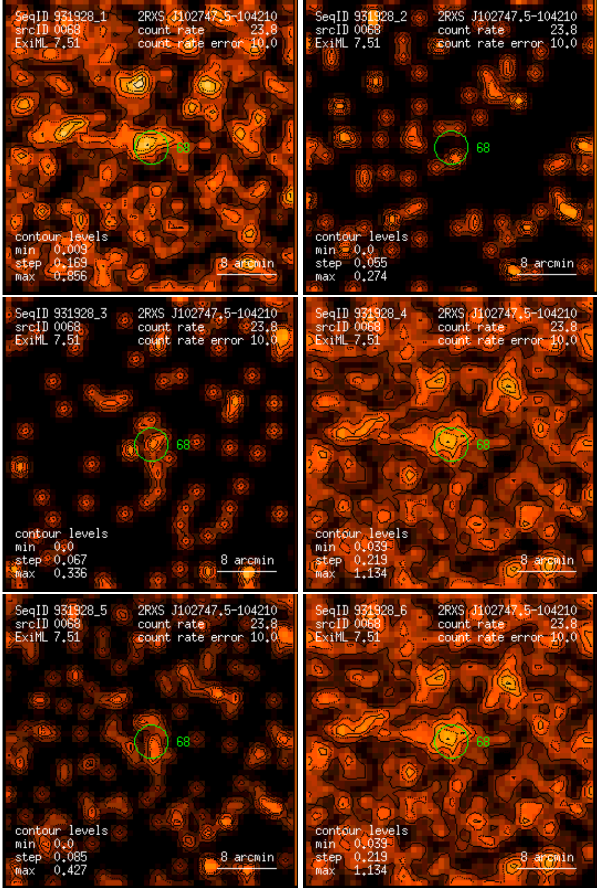
Figure 68: RASS 931928: detection 0068: band rate images, Gaussian filter: (1) PSPC channels 11 – 41, (2) 52 – 90, (3) 91 – 201, (4) 11 – 235, (5) 52 – 201, (6) 11 – 201. Broad band rates in counts/ks. Band rate contour levels in counts/ks/arcmin 2 .
