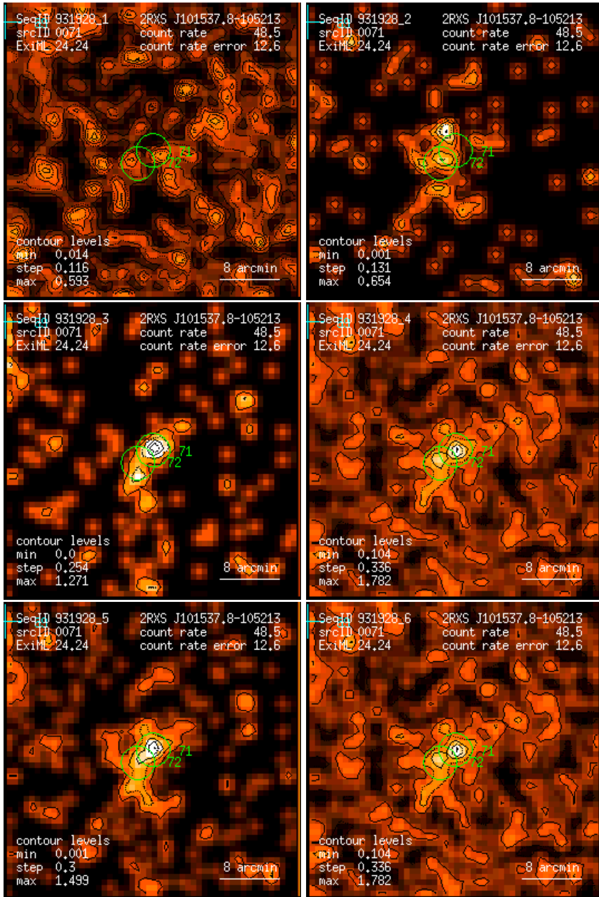
Figure 71: RASS 931928: detection 0071: band rate images, Gaussian filter: (1) PSPC channels 11 – 41, (2) 52 – 90, (3) 91 – 201, (4) 11 – 235, (5) 52 – 201, (6) 11 – 201. Broad band rates in counts/ks. Band rate contour levels in counts/ks/arcmin 2 .
