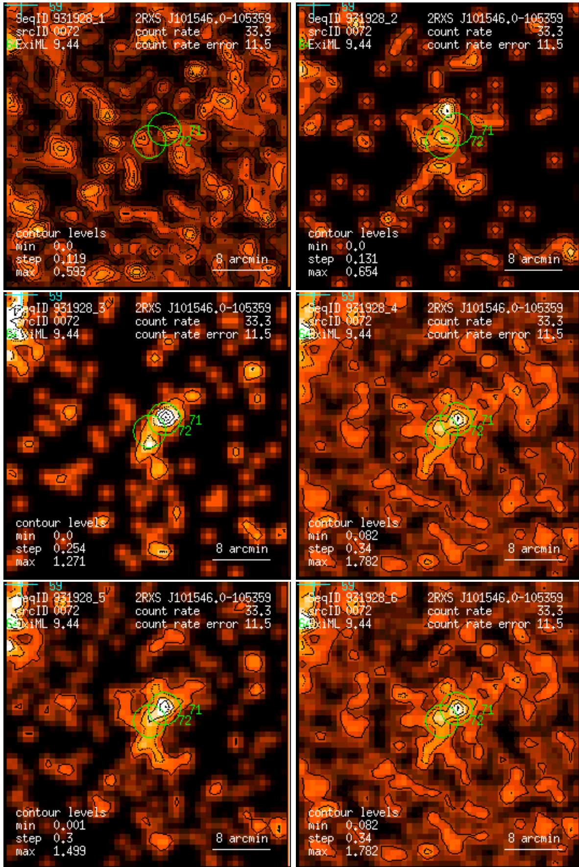
Figure 72: RASS 931928: detection 0072: band rate images, Gaussian filter: (1) PSPC channels 11 – 41, (2) 52 – 90, (3) 91 – 201, (4) 11 – 235, (5) 52 – 201, (6) 11 – 201. Broad band rates in counts/ks. Band rate contour levels in counts/ks/arcmin 2 .
