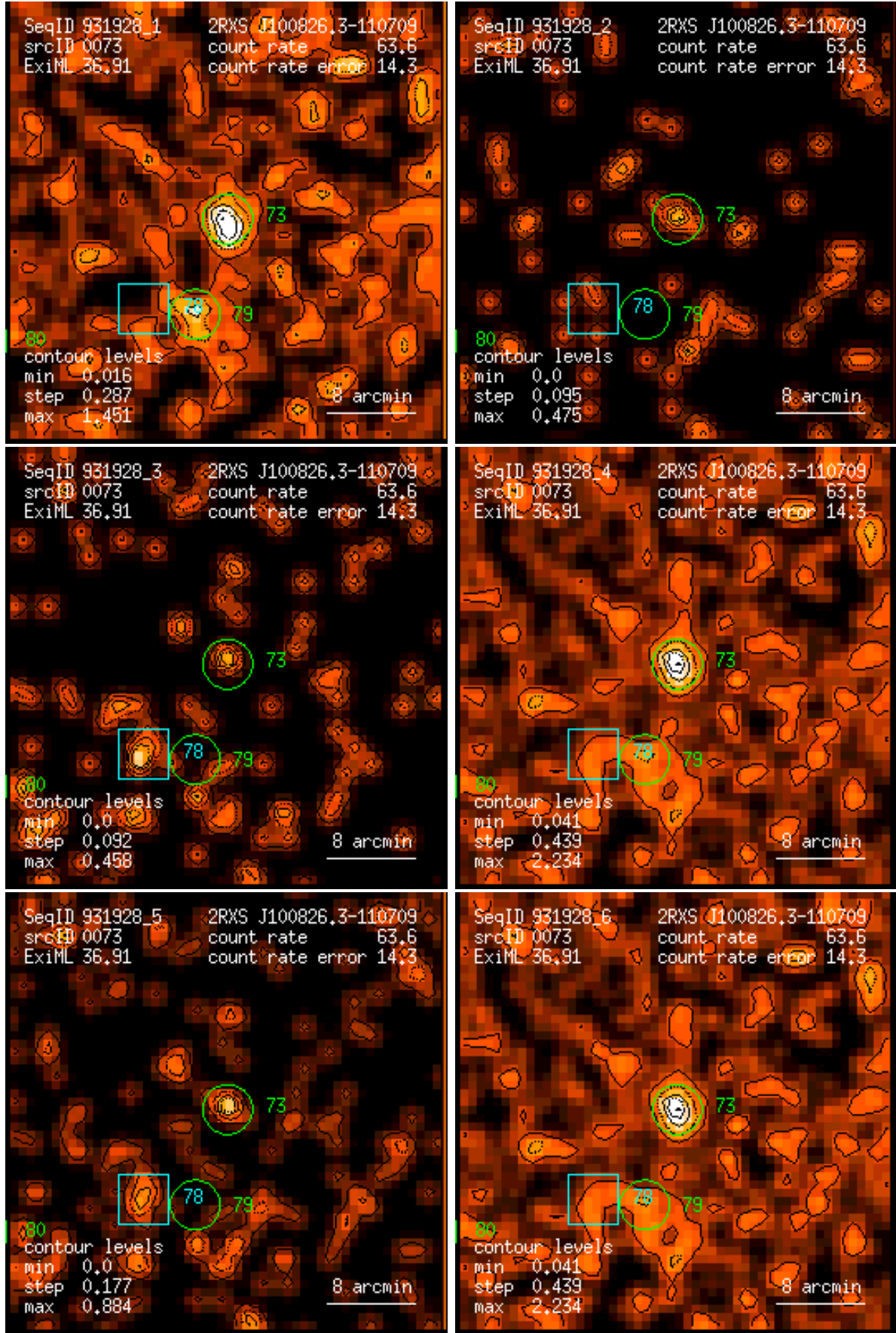
Figure 73: RASS 931928: detection 0073: band rate images, Gaussian filter: (1) PSPC channels 11 – 41, (2) 52 – 90, (3) 91 – 201, (4) 11 – 235, (5) 52 – 201, (6) 11 – 201. Broad band rates in counts/ks. Band rate contour levels in counts/ks/arcmin 2 .
