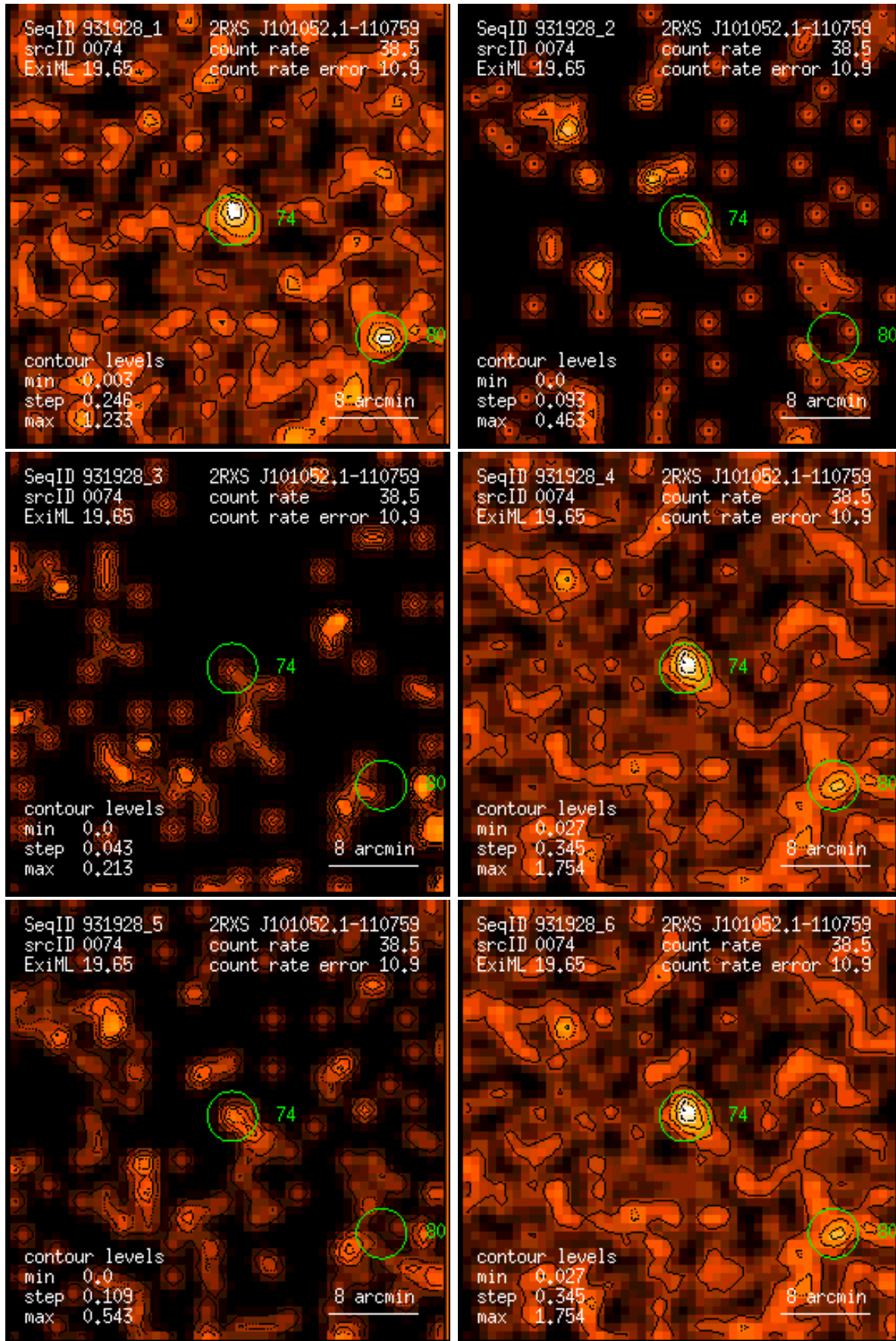
Figure 74: RASS 931928: detection 0074: band rate images, Gaussian filter: (1) PSPC channels 11 – 41, (2) 52 – 90, (3) 91 – 201, (4) 11 – 235, (5) 52 – 201, (6) 11 – 201. Broad band rates in counts/ks. Band rate contour levels in counts/ks/arcmin 2 .
