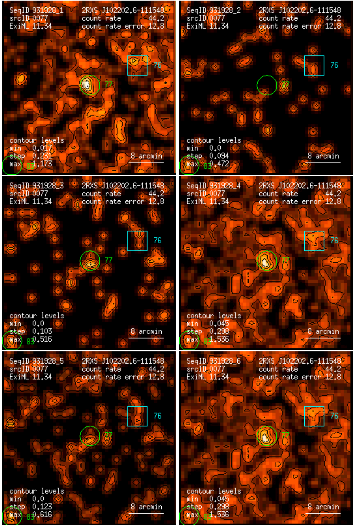
Figure 77: RASS 931928: detection 0077: band rate images, Gaussian filter: (1) PSPC channels 11 – 41, (2) 52 – 90, (3) 91 – 201, (4) 11 – 235, (5) 52 – 201, (6) 11 – 201. Broad band rates in counts/ks. Band rate contour levels in counts/ks/arcmin 2 .
