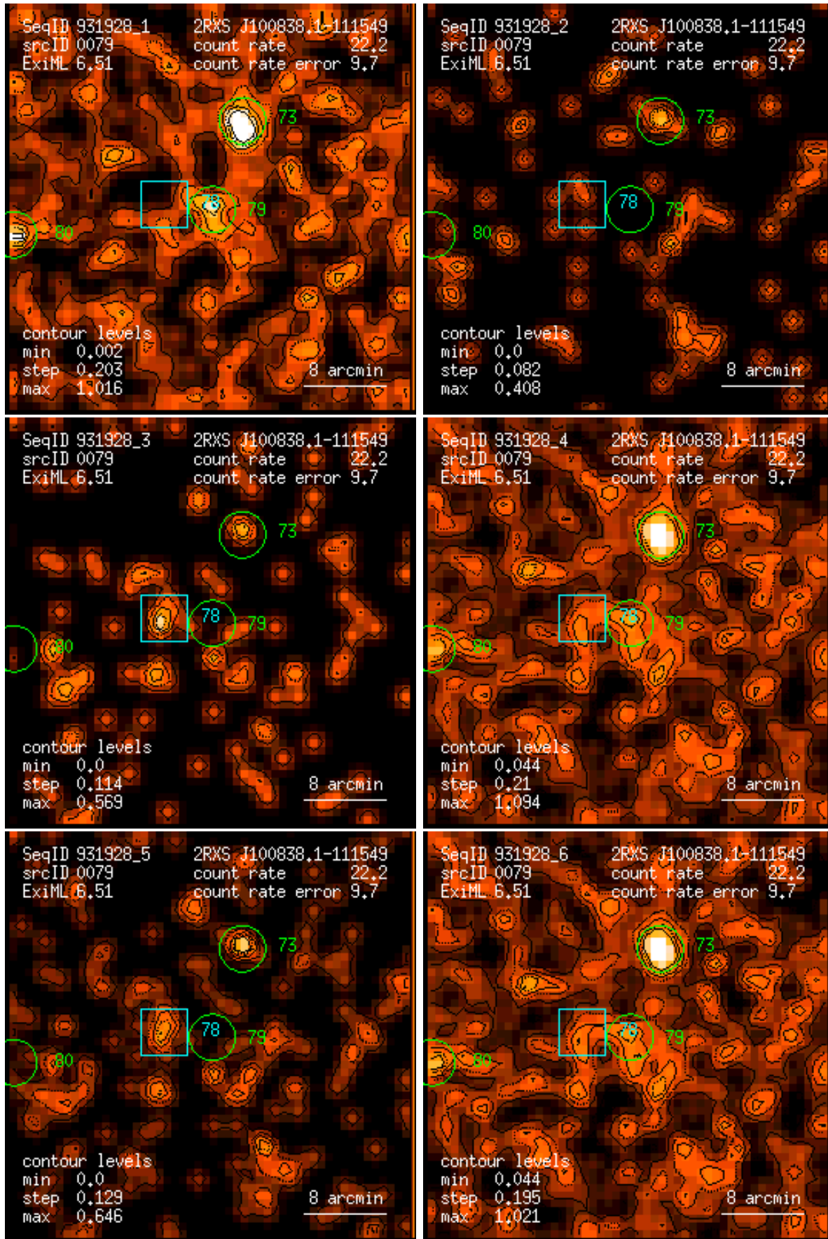
Figure 79: RASS 931928: detection 0079: band rate images, Gaussian filter: (1) PSPC channels 11 – 41, (2) 52 – 90, (3) 91 – 201, (4) 11 – 235, (5) 52 – 201, (6) 11 – 201. Broad band rates in counts/ks. Band rate contour levels in counts/ks/arcmin 2 .
