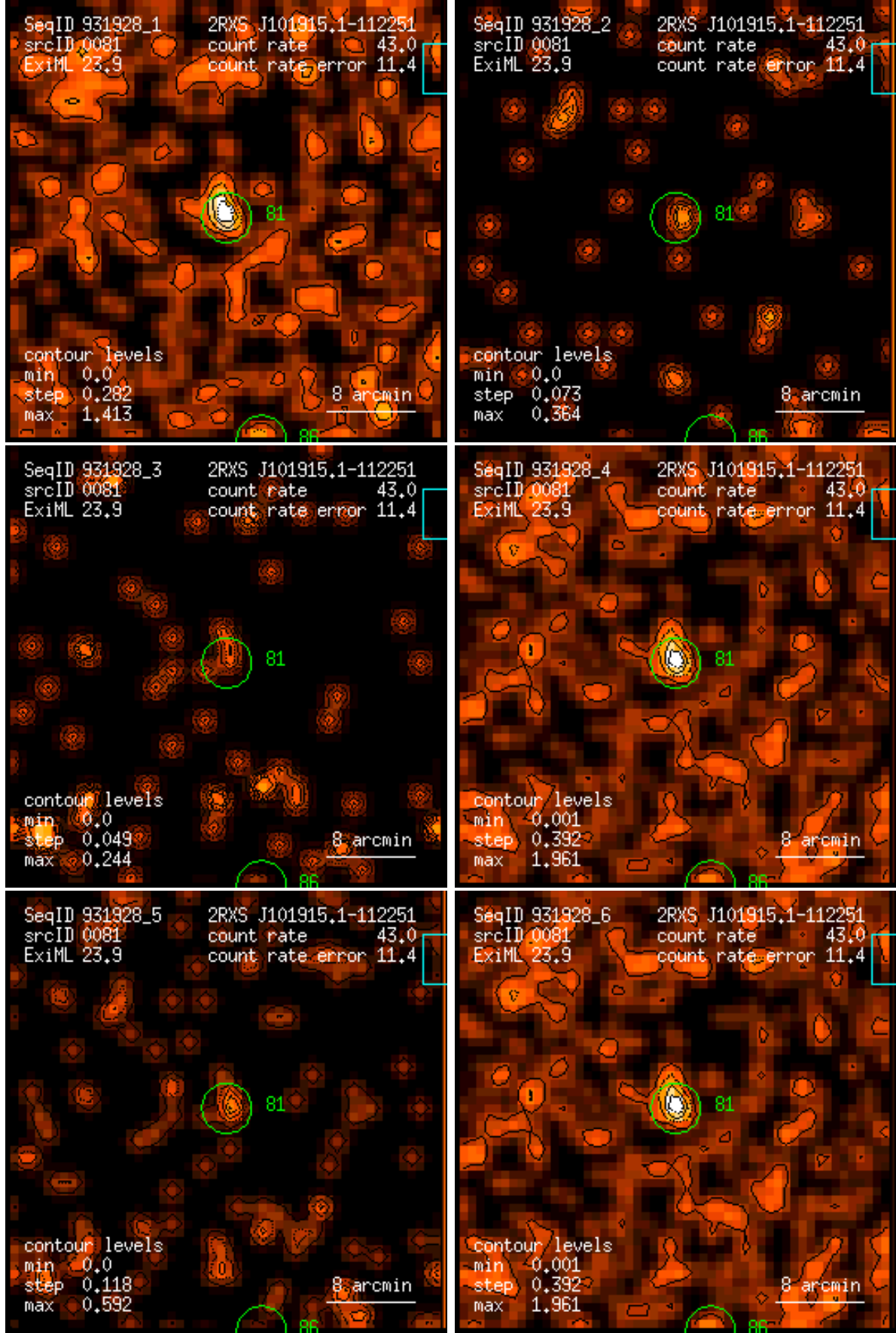
Figure 81: RASS 931928: detection 0081: band rate images, Gaussian filter: (1) PSPC channels 11 – 41, (2) 52 – 90, (3) 91 – 201, (4) 11 – 235, (5) 52 – 201, (6) 11 – 201. Broad band rates in counts/ks. Band rate contour levels in counts/ks/arcmin 2 .
