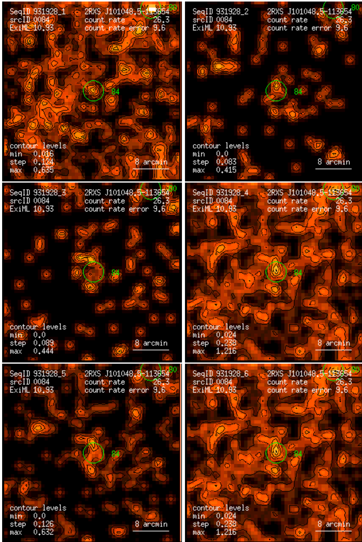
Figure 84: RASS 931928: detection 0084: band rate images, Gaussian filter: (1) PSPC channels 11 – 41, (2) 52 – 90, (3) 91 – 201, (4) 11 – 235, (5) 52 – 201, (6) 11 – 201. Broad band rates in counts/ks. Band rate contour levels in counts/ks/arcmin 2 .
