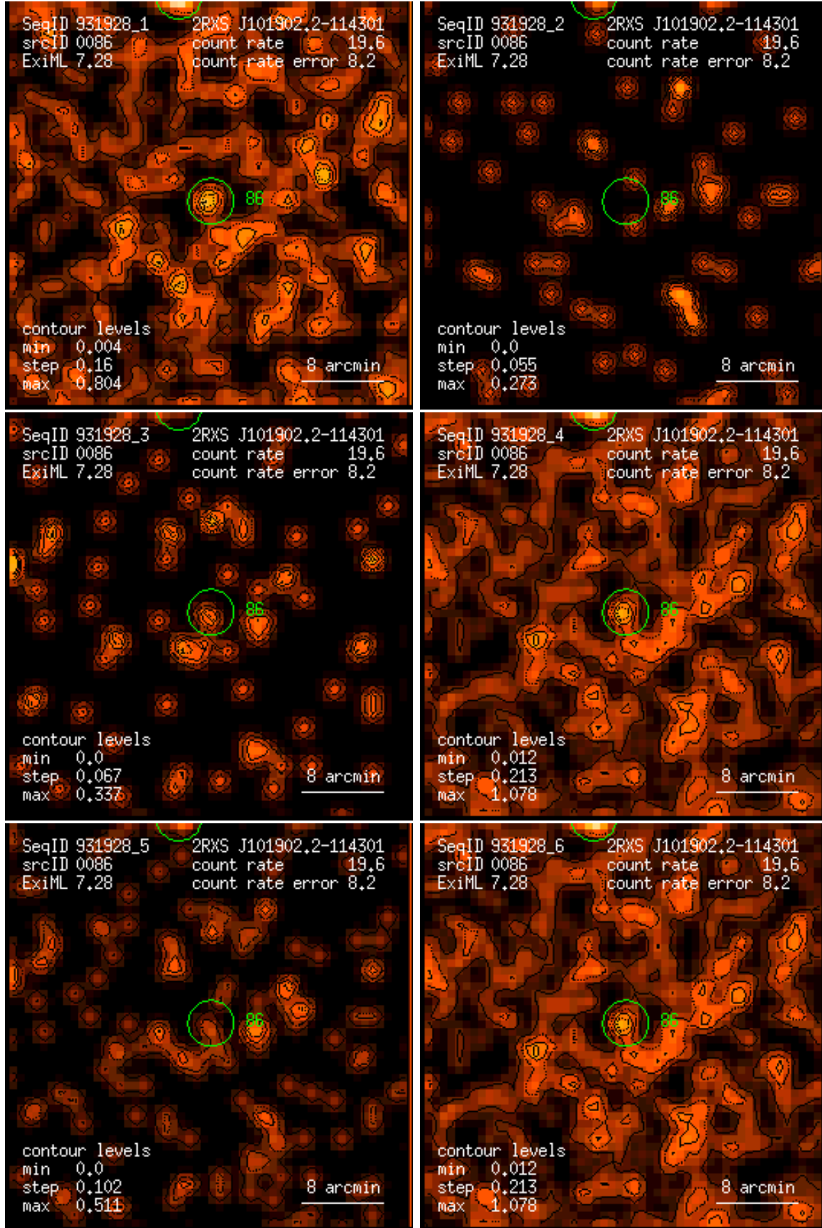
Figure 86: RASS 931928: detection 0086: band rate images, Gaussian filter: (1) PSPC channels 11 – 41, (2) 52 – 90, (3) 91 – 201, (4) 11 – 235, (5) 52 – 201, (6) 11 – 201. Broad band rates in counts/ks. Band rate contour levels in counts/ks/arcmin 2 .
