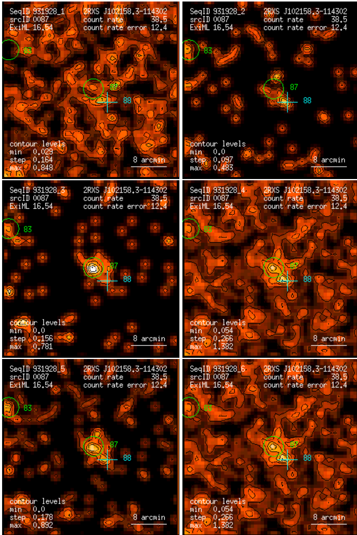
Figure 87: RASS 931928: detection 0087: band rate images, Gaussian filter: (1) PSPC channels 11 – 41, (2) 52 – 90, (3) 91 – 201, (4) 11 – 235, (5) 52 – 201, (6) 11 – 201. Broad band rates in counts/ks. Band rate contour levels in counts/ks/arcmin 2 .
