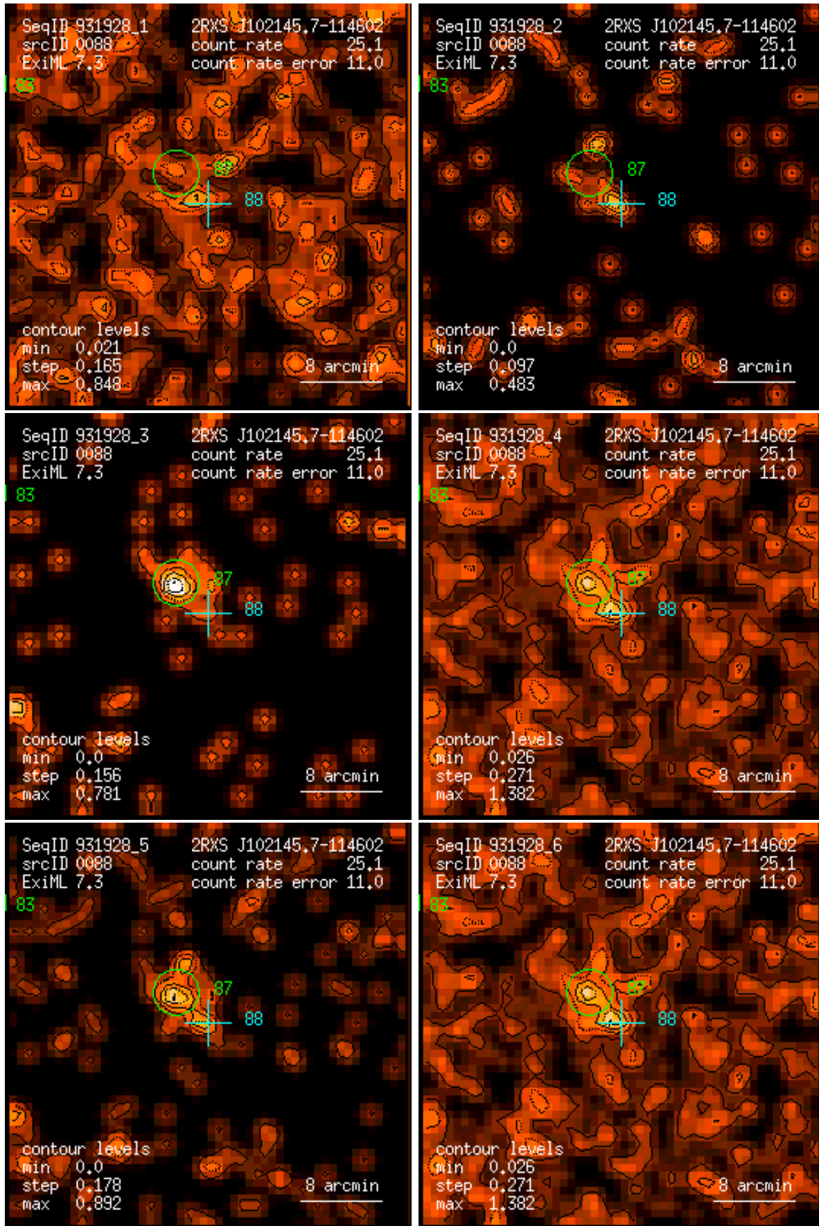
Figure 88: RASS 931928: detection 0088: band rate images, Gaussian filter: (1) PSPC channels 11 – 41, (2) 52 – 90, (3) 91 – 201, (4) 11 – 235, (5) 52 – 201, (6) 11 – 201. Broad band rates in counts/ks. Band rate contour levels in counts/ks/arcmin 2 .
