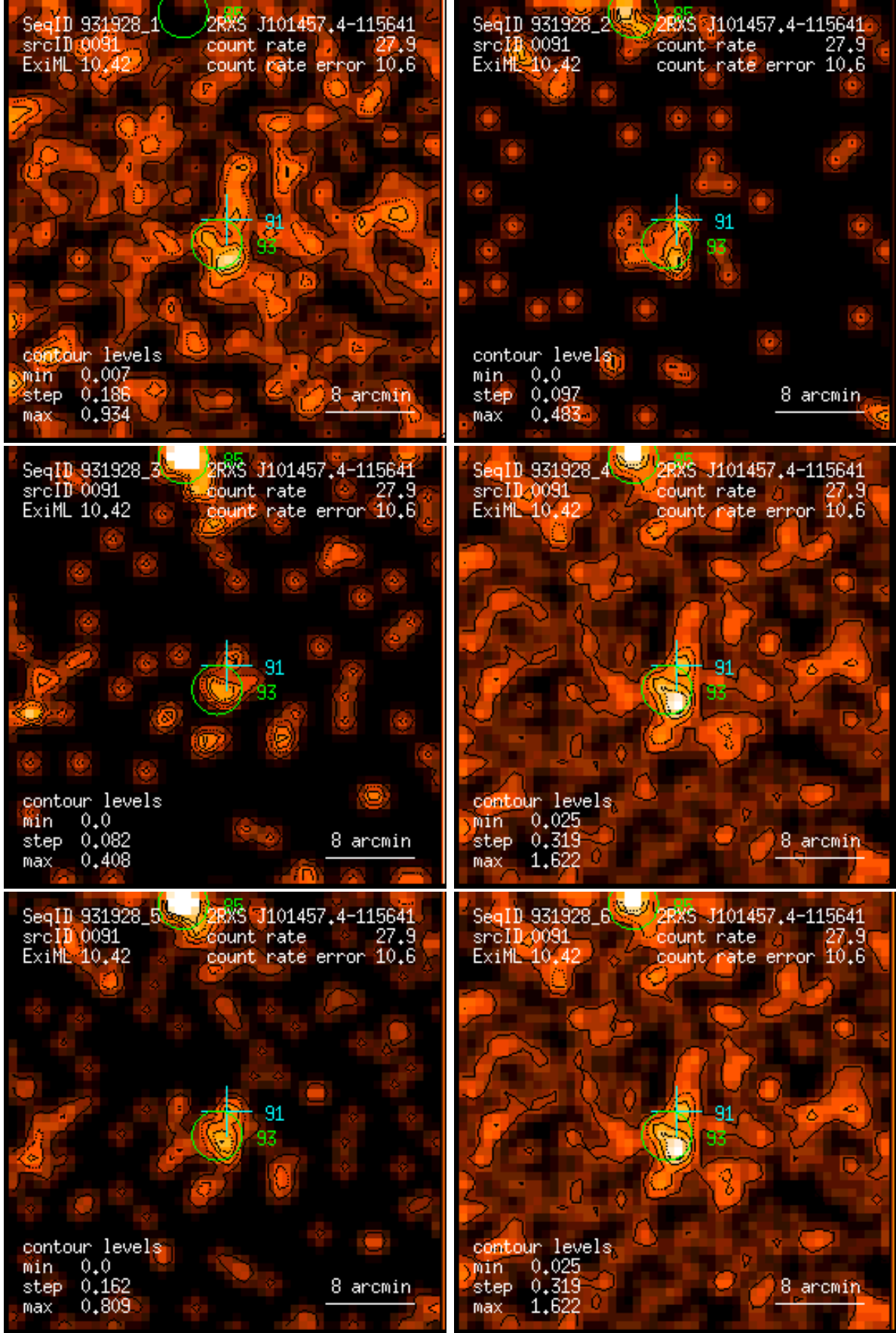
Figure 91: RASS 931928: detection 0091: band rate images, Gaussian filter: (1) PSPC channels 11 – 41, (2) 52 – 90, (3) 91 – 201, (4) 11 – 235, (5) 52 – 201, (6) 11 – 201. Broad band rates in counts/ks. Band rate contour levels in counts/ks/arcmin 2 .
