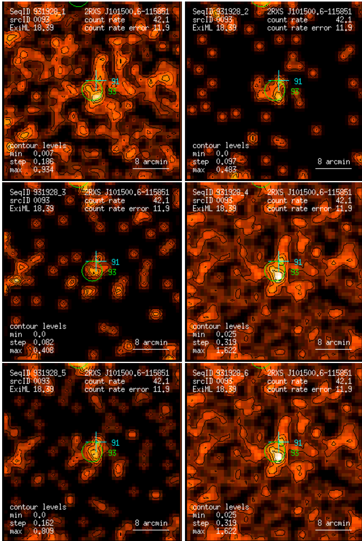
Figure 93: RASS 931928: detection 0093: band rate images, Gaussian filter: (1) PSPC channels 11 – 41, (2) 52 – 90, (3) 91 – 201, (4) 11 – 235, (5) 52 – 201, (6) 11 – 201. Broad band rates in counts/ks. Band rate contour levels in counts/ks/arcmin 2 .
