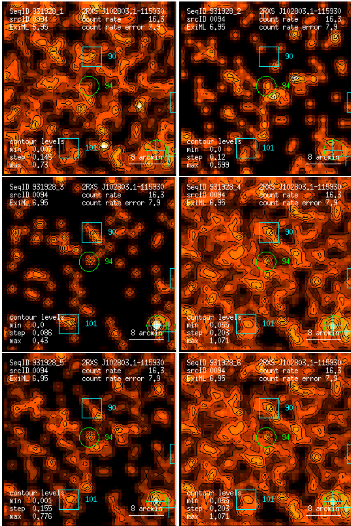
Figure 94: RASS 931928: detection 0094: band rate images, Gaussian filter: (1) PSPC channels 11 – 41, (2) 52 – 90, (3) 91 – 201, (4) 11 – 235, (5) 52 – 201, (6) 11 – 201. Broad band rates in counts/ks. Band rate contour levels in counts/ks/arcmin 2 .
