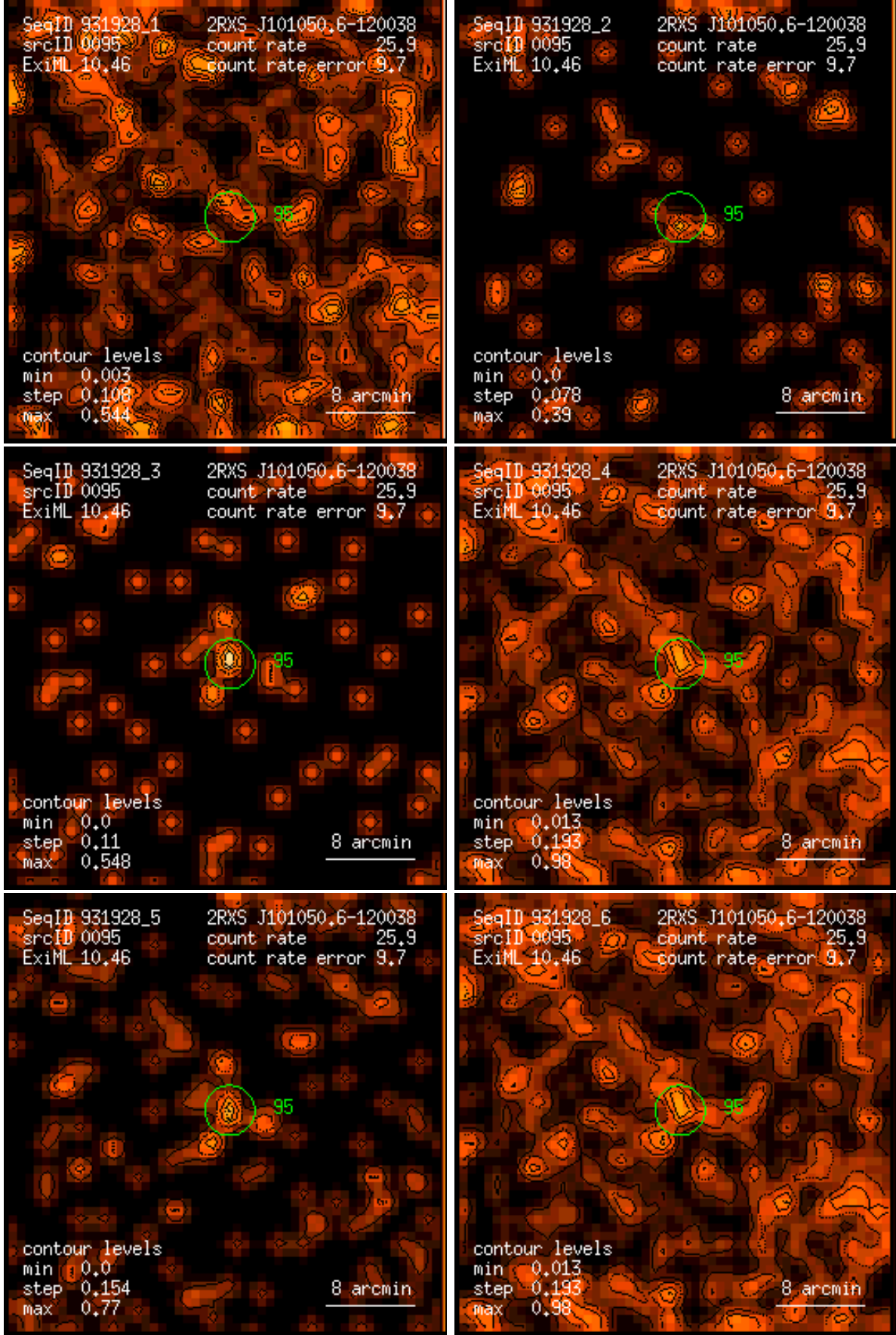
Figure 95: RASS 931928: detection 0095: band rate images, Gaussian filter: (1) PSPC channels 11 – 41, (2) 52 – 90, (3) 91 – 201, (4) 11 – 235, (5) 52 – 201, (6) 11 – 201. Broad band rates in counts/ks. Band rate contour levels in counts/ks/arcmin 2 .
