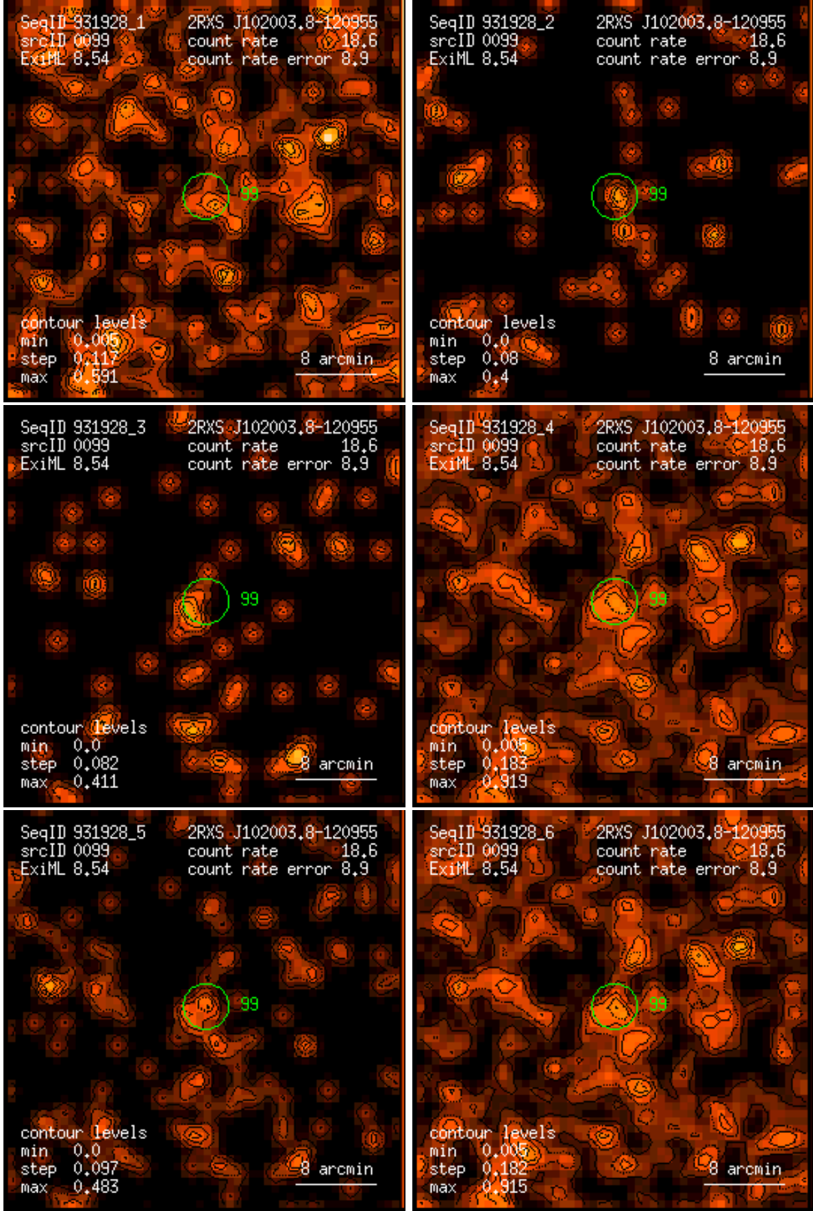
Figure 99: RASS 931928: detection 0099: band rate images, Gaussian filter: (1) PSPC channels 11 – 41, (2) 52 – 90, (3) 91 – 201, (4) 11 – 235, (5) 52 – 201, (6) 11 – 201. Broad band rates in counts/ks. Band rate contour levels in counts/ks/arcmin 2 .
