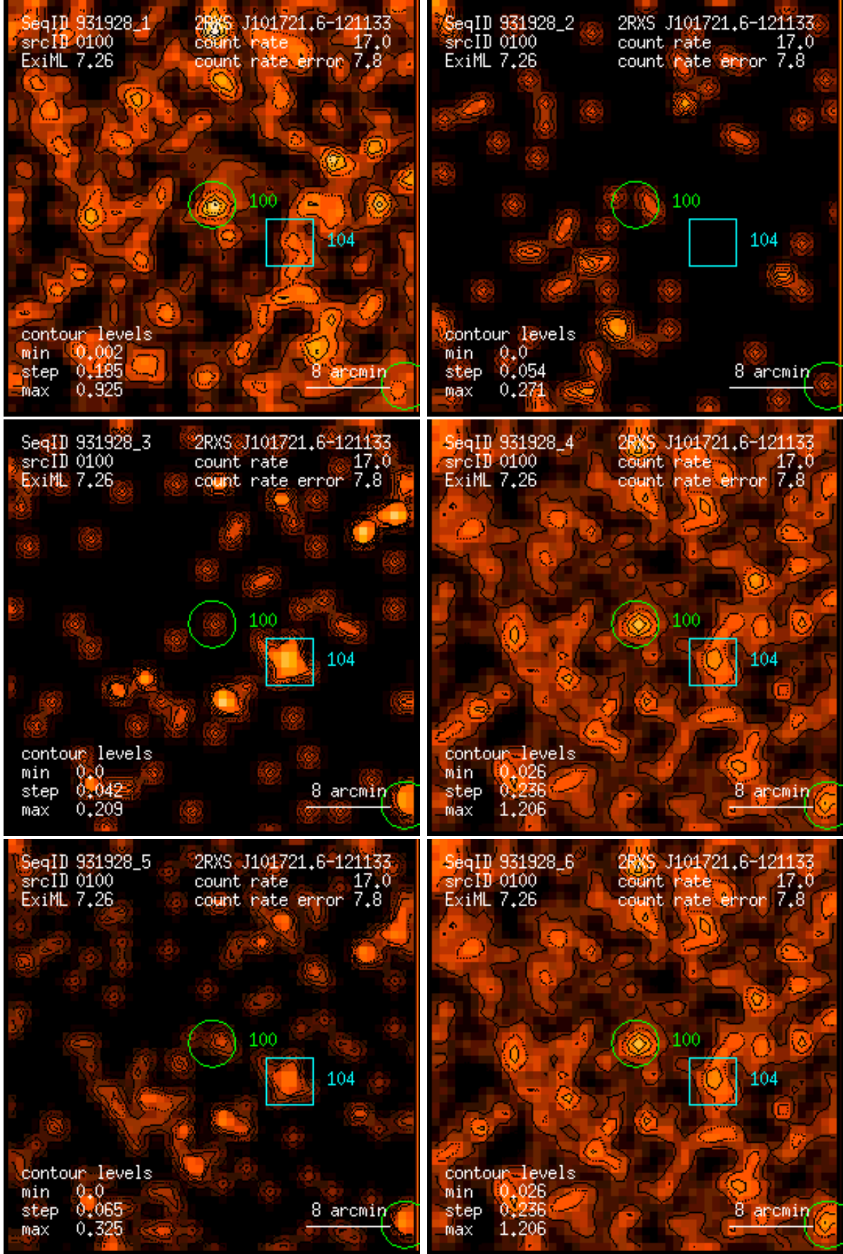
Figure 100: RASS 931928: detection 0100: band rate images, Gaussian filter: (1) PSPC channels 11 – 41, (2) 52 – 90, (3) 91 – 201, (4) 11 – 235, (5) 52 – 201, (6) 11 – 201. Broad band rates in counts/ks. Band rate contour levels in counts/ks/arcmin 2 .
