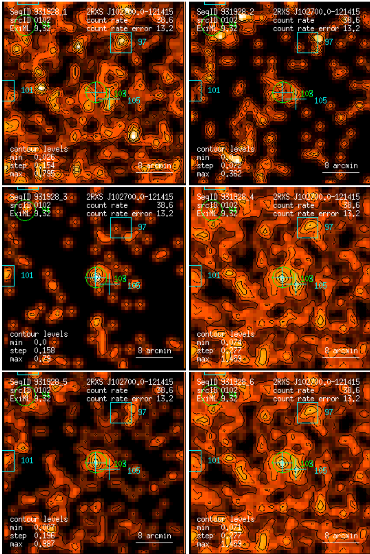
Figure 102: RASS 931928: detection 0102: band rate images, Gaussian filter: (1) PSPC channels 11 – 41, (2) 52 – 90, (3) 91 – 201, (4) 11 – 235, (5) 52 – 201, (6) 11 – 201. Broad band rates in counts/ks. Band rate contour levels in counts/ks/arcmin 2 .
