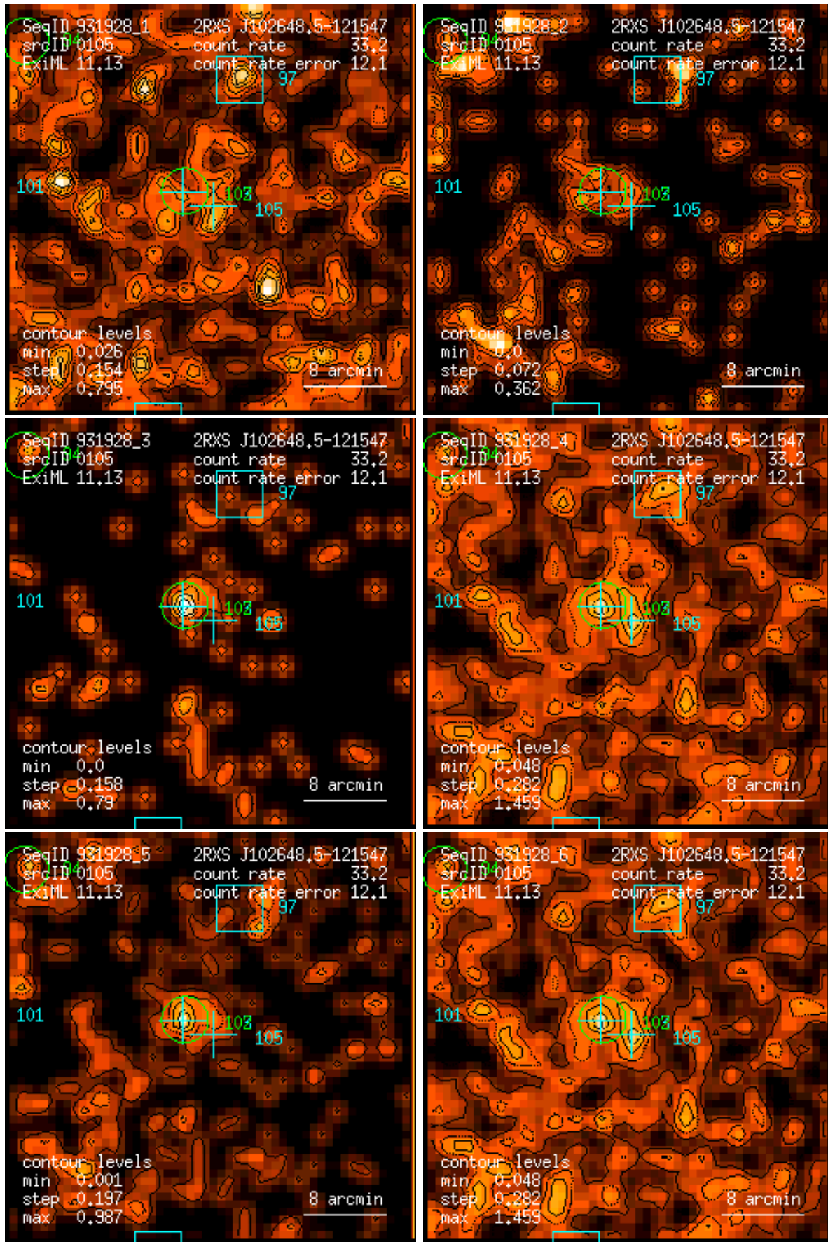
Figure 105: RASS 931928: detection 0105: band rate images, Gaussian filter: (1) PSPC channels 11 – 41, (2) 52 – 90, (3) 91 – 201, (4) 11 – 235, (5) 52 – 201, (6) 11 – 201. Broad band rates in counts/ks. Band rate contour levels in counts/ks/arcmin 2 .
