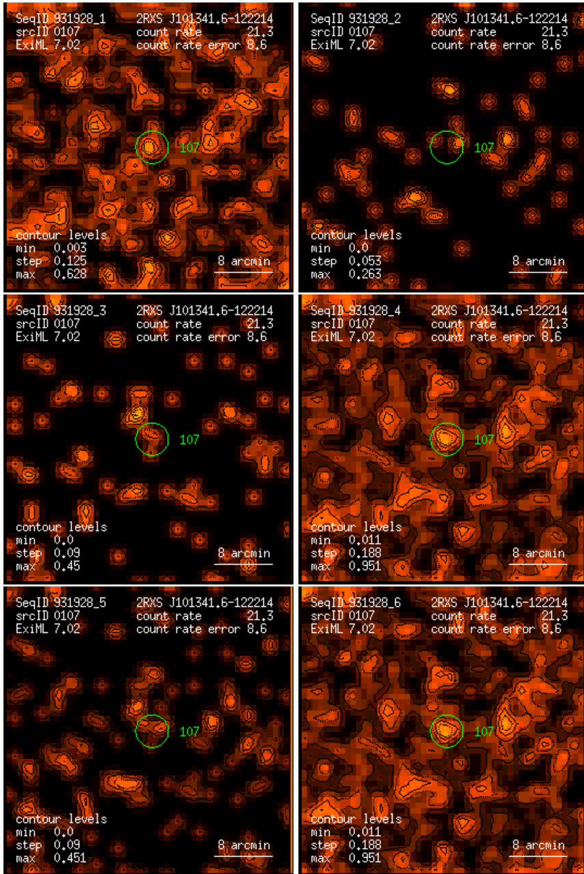
Figure 107: RASS 931928: detection 0107: band rate images, Gaussian filter: (1) PSPC channels 11 – 41, (2) 52 – 90, (3) 91 – 201, (4) 11 – 235, (5) 52 – 201, (6) 11 – 201. Broad band rates in counts/ks. Band rate contour levels in counts/ks/arcmin 2 .
