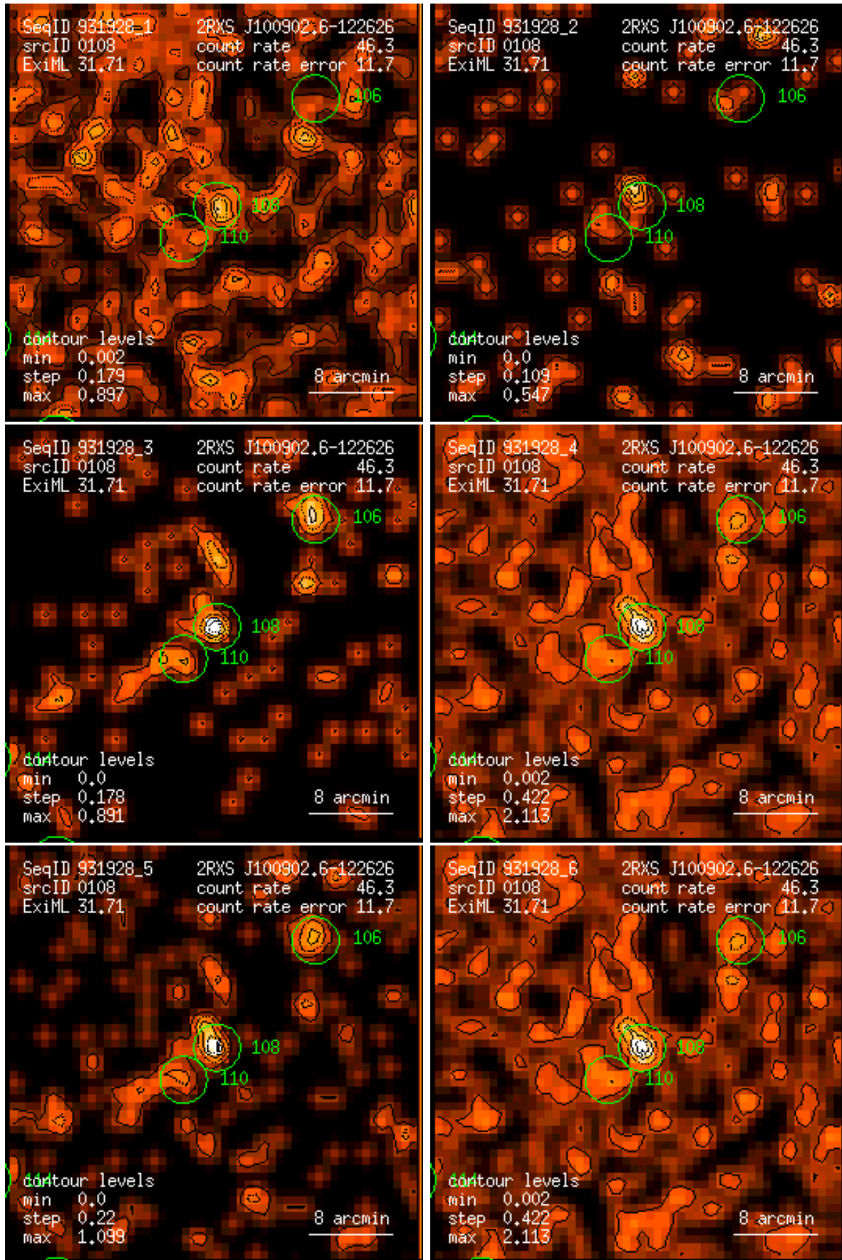
Figure 108: RASS 931928: detection 0108: band rate images, Gaussian filter: (1) PSPC channels 11 – 41, (2) 52 – 90, (3) 91 – 201, (4) 11 – 235, (5) 52 – 201, (6) 11 – 201. Broad band rates in counts/ks. Band rate contour levels in counts/ks/arcmin 2 .
