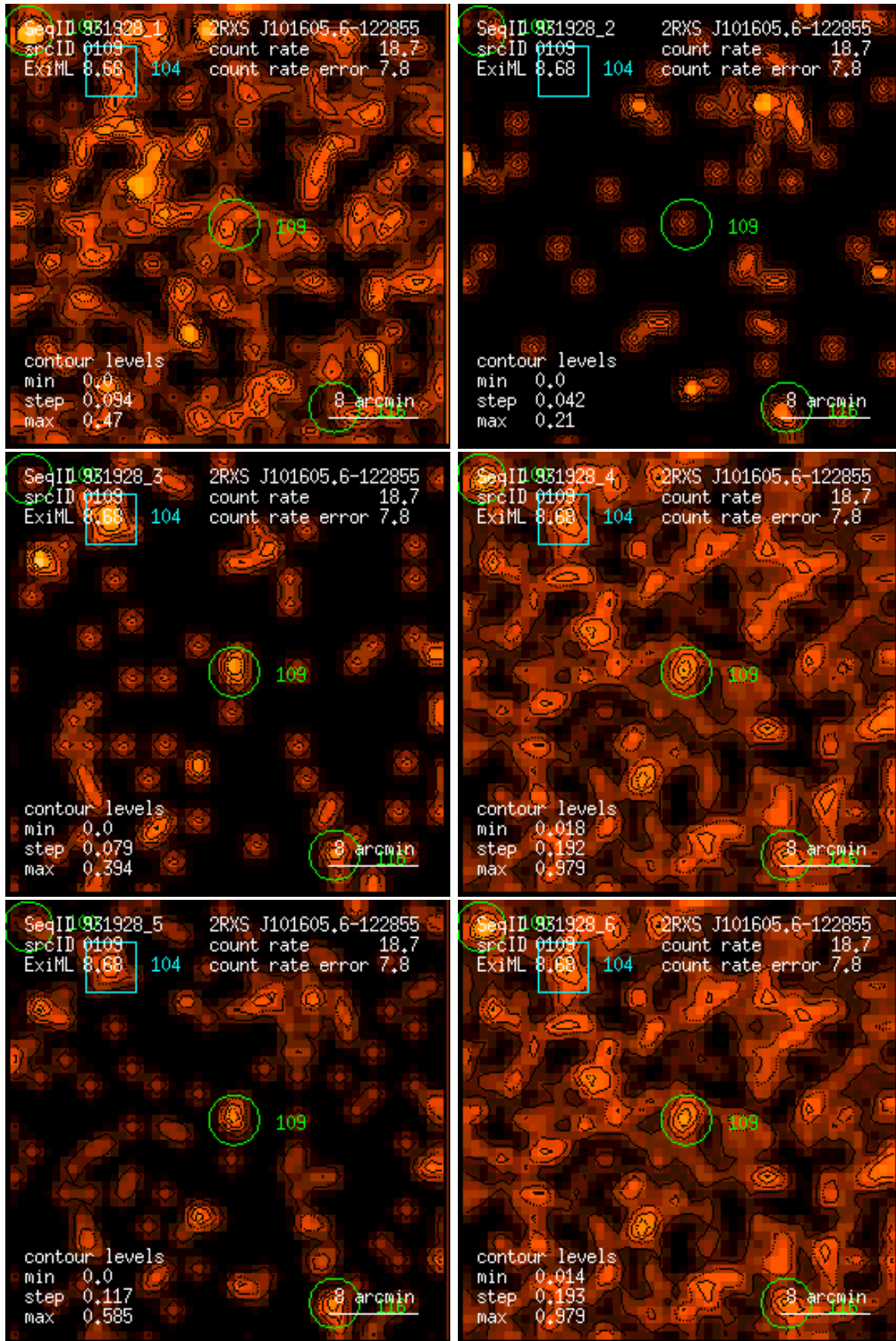
Figure 109: RASS 931928: detection 0109: band rate images, Gaussian filter: (1) PSPC channels 11 – 41, (2) 52 – 90, (3) 91 – 201, (4) 11 – 235, (5) 52 – 201, (6) 11 – 201. Broad band rates in counts/ks. Band rate contour levels in counts/ks/arcmin 2 .
