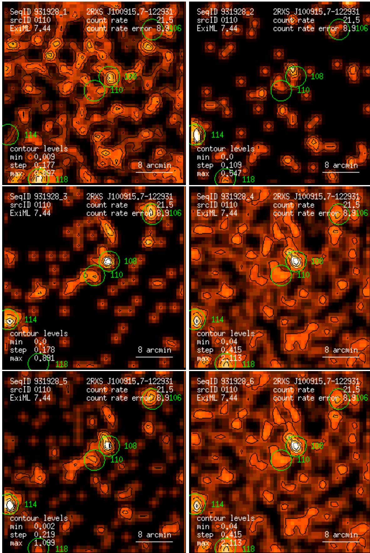
Figure 110: RASS 931928: detection 0110: band rate images, Gaussian filter: (1) PSPC channels 11 – 41, (2) 52 – 90, (3) 91 – 201, (4) 11 – 235, (5) 52 – 201, (6) 11 – 201. Broad band rates in counts/ks. Band rate contour levels in counts/ks/arcmin 2 .
