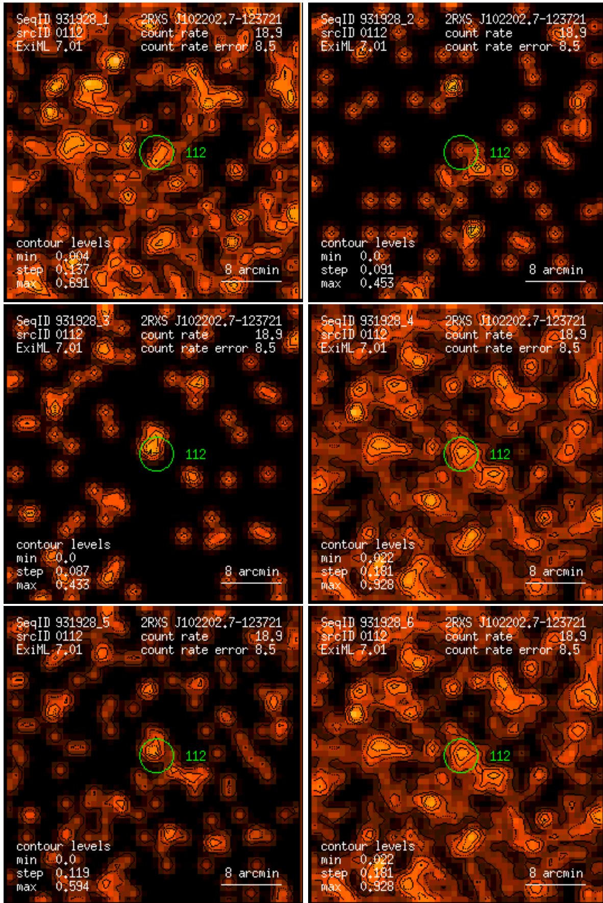
Figure 112: RASS 931928: detection 0112: band rate images, Gaussian filter: (1) PSPC channels 11 – 41, (2) 52 – 90, (3) 91 – 201, (4) 11 – 235, (5) 52 – 201, (6) 11 – 201. Broad band rates in counts/ks. Band rate contour levels in counts/ks/arcmin 2 .
