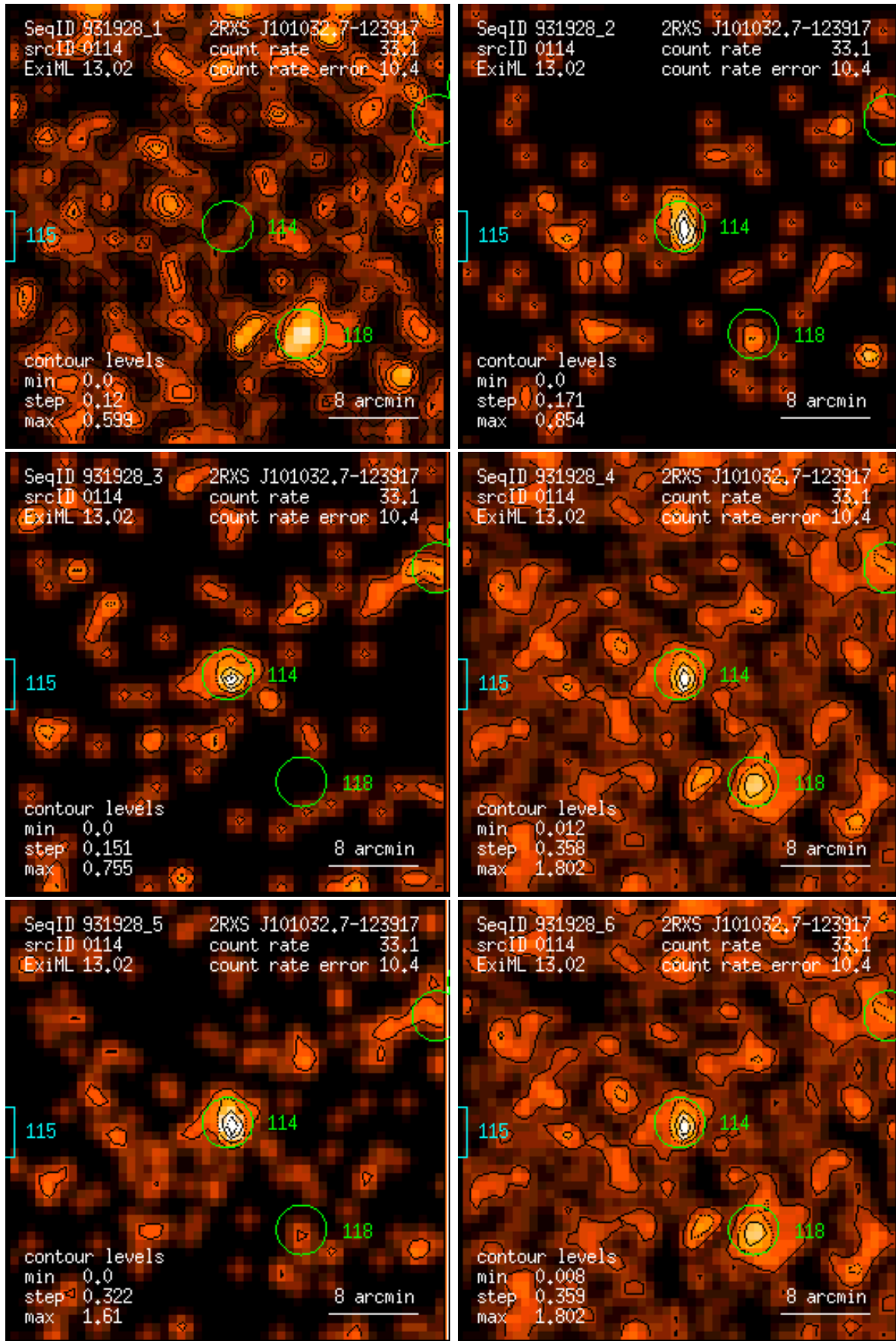
Figure 114: RASS 931928: detection 0114: band rate images, Gaussian filter: (1) PSPC channels 11 – 41, (2) 52 – 90, (3) 91 – 201, (4) 11 – 235, (5) 52 – 201, (6) 11 – 201. Broad band rates in counts/ks. Band rate contour levels in counts/ks/arcmin 2 .
