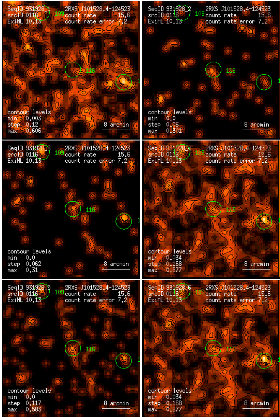
Figure 116: RASS 931928: detection 0116: band rate images, Gaussian filter: (1) PSPC channels 11 – 41, (2) 52 – 90, (3) 91 – 201, (4) 11 – 235, (5) 52 – 201, (6) 11 – 201. Broad band rates in counts/ks. Band rate contour levels in counts/ks/arcmin 2 .
