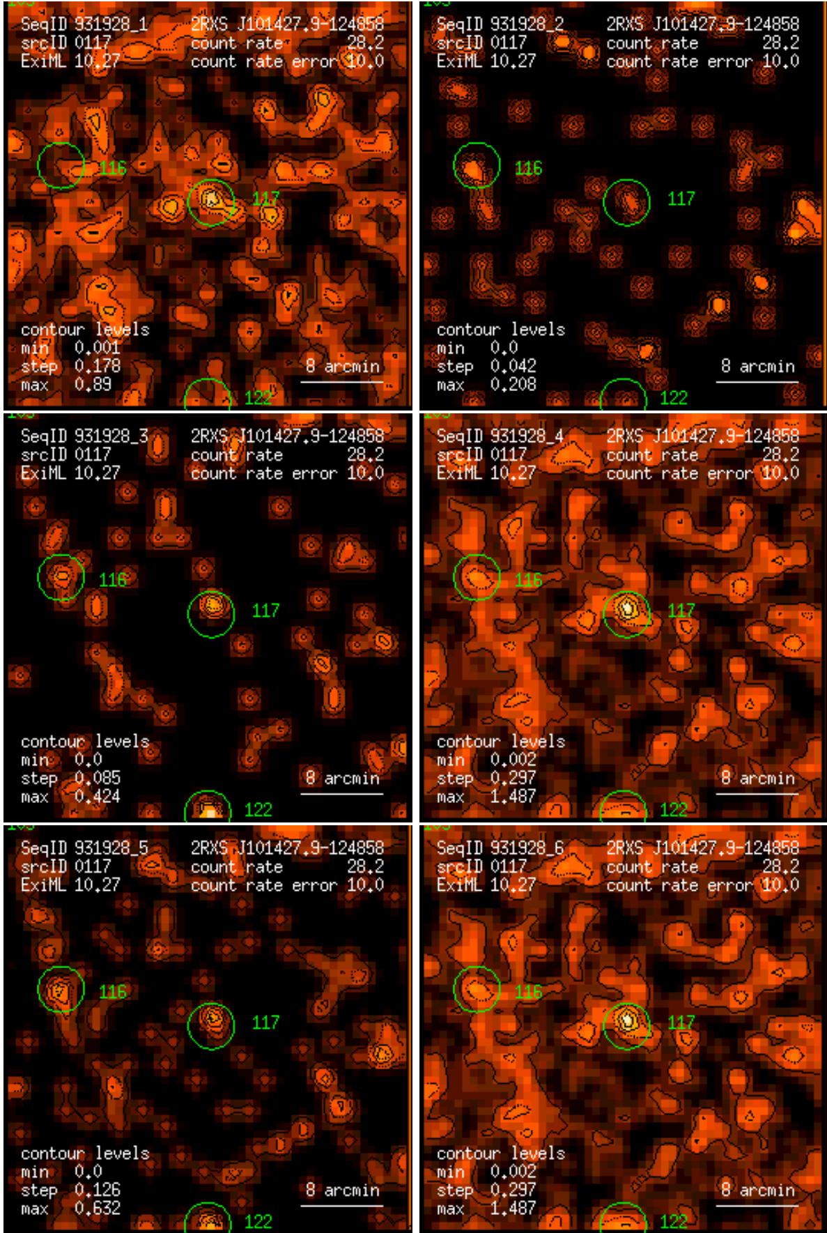
Figure 117: RASS 931928: detection 0117: band rate images, Gaussian filter: (1) PSPC channels 11 – 41, (2) 52 – 90, (3) 91 – 201, (4) 11 – 235, (5) 52 – 201, (6) 11 – 201. Broad band rates in counts/ks. Band rate contour levels in counts/ks/arcmin 2 .
