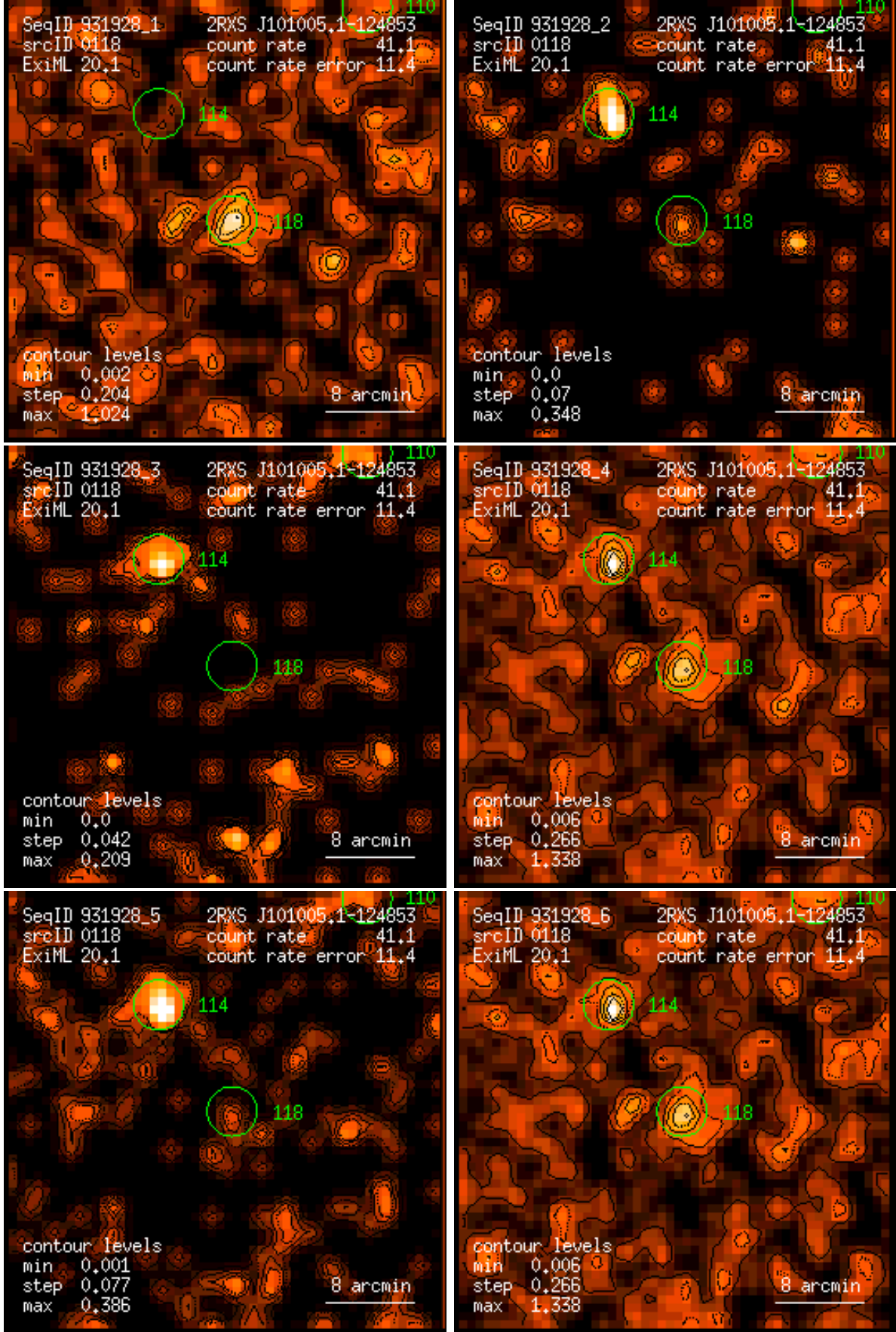
Figure 118: RASS 931928: detection 0118: band rate images, Gaussian filter: (1) PSPC channels 11 – 41, (2) 52 – 90, (3) 91 – 201, (4) 11 – 235, (5) 52 – 201, (6) 11 – 201. Broad band rates in counts/ks. Band rate contour levels in counts/ks/arcmin 2 .
