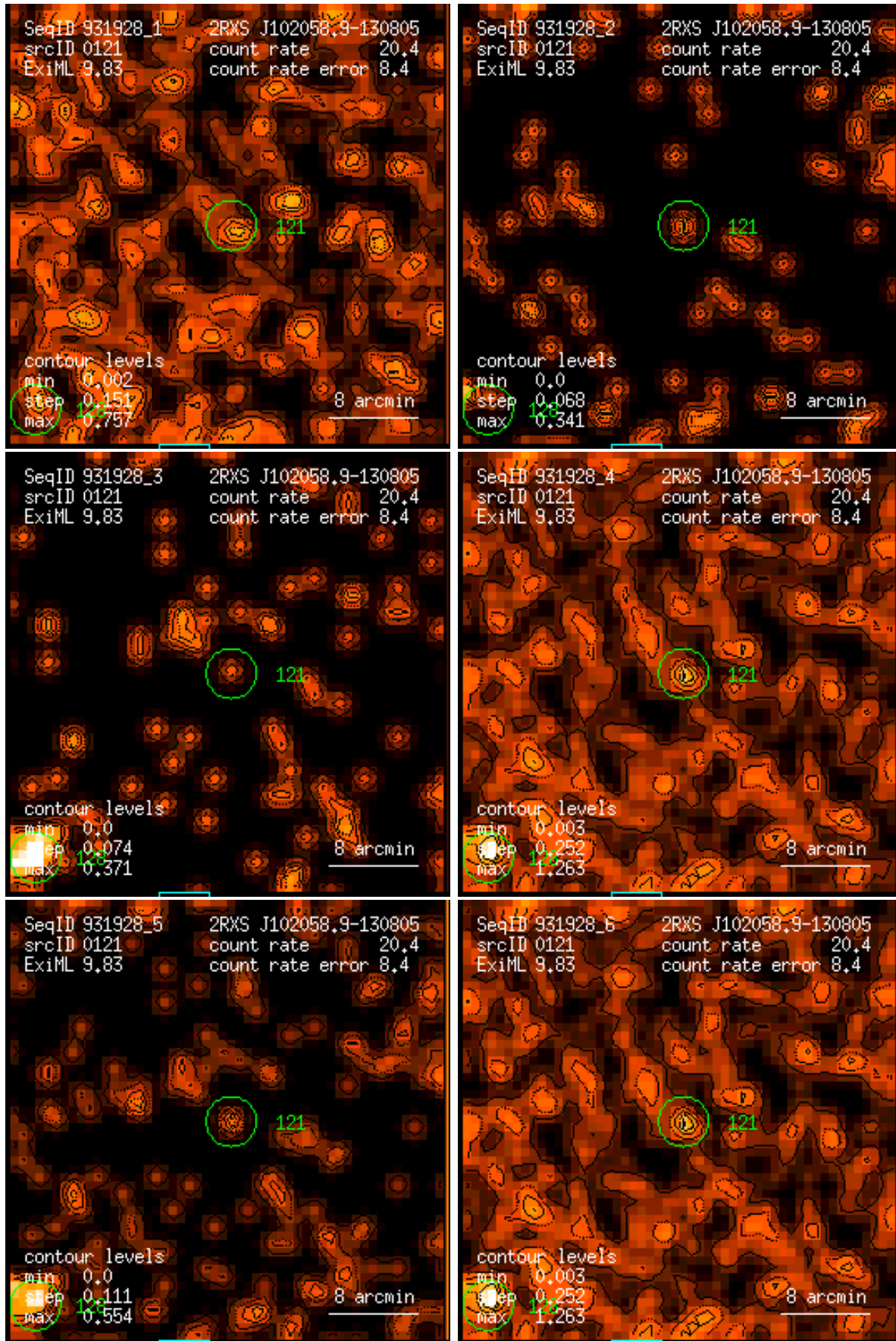
Figure 121: RASS 931928: detection 0121: band rate images, Gaussian filter: (1) PSPC channels 11 – 41, (2) 52 – 90, (3) 91 – 201, (4) 11 – 235, (5) 52 – 201, (6) 11 – 201. Broad band rates in counts/ks. Band rate contour levels in counts/ks/arcmin 2 .
