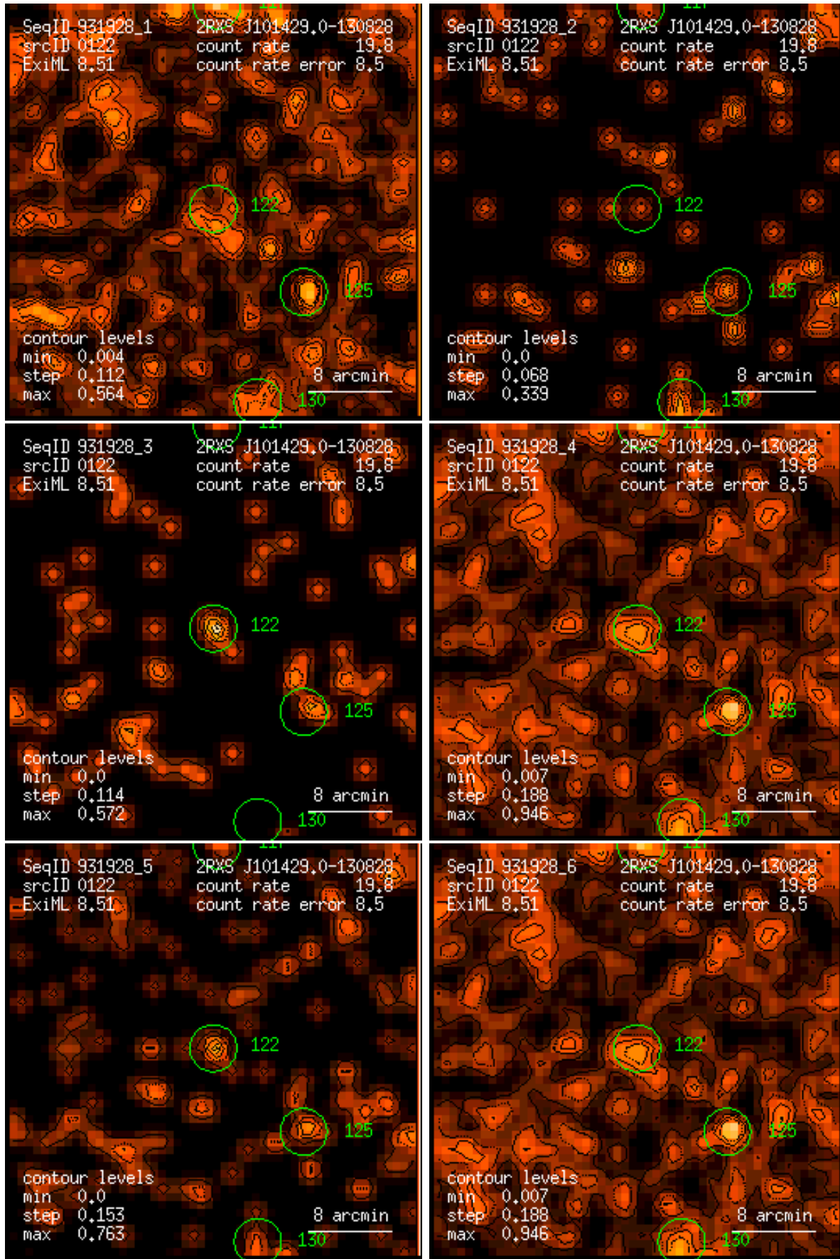
Figure 122: RASS 931928: detection 0122: band rate images, Gaussian filter: (1) PSPC channels 11 – 41, (2) 52 – 90, (3) 91 – 201, (4) 11 – 235, (5) 52 – 201, (6) 11 – 201. Broad band rates in counts/ks. Band rate contour levels in counts/ks/arcmin 2 .
