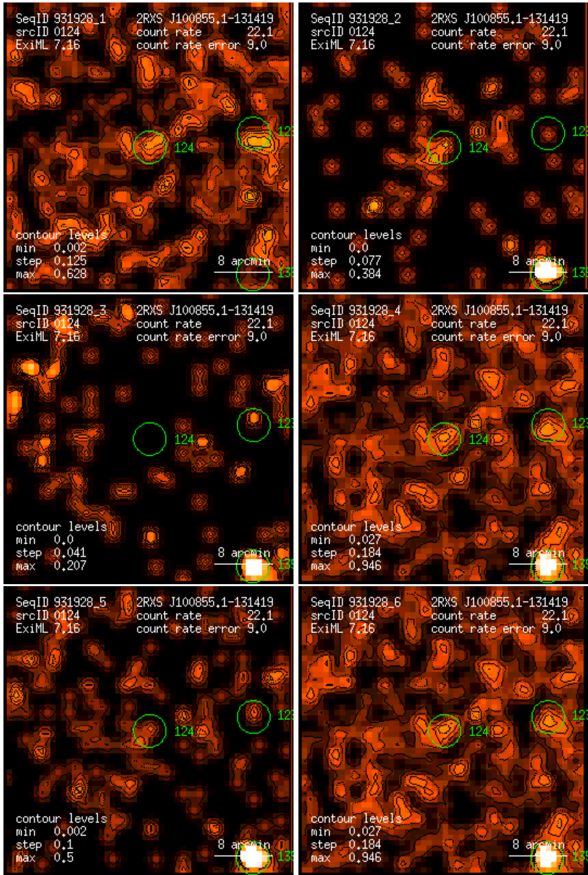
Figure 124: RASS 931928: detection 0124: band rate images, Gaussian filter: (1) PSPC channels 11 – 41, (2) 52 – 90, (3) 91 – 201, (4) 11 – 235, (5) 52 – 201, (6) 11 – 201. Broad band rates in counts/ks. Band rate contour levels in counts/ks/arcmin 2 .
