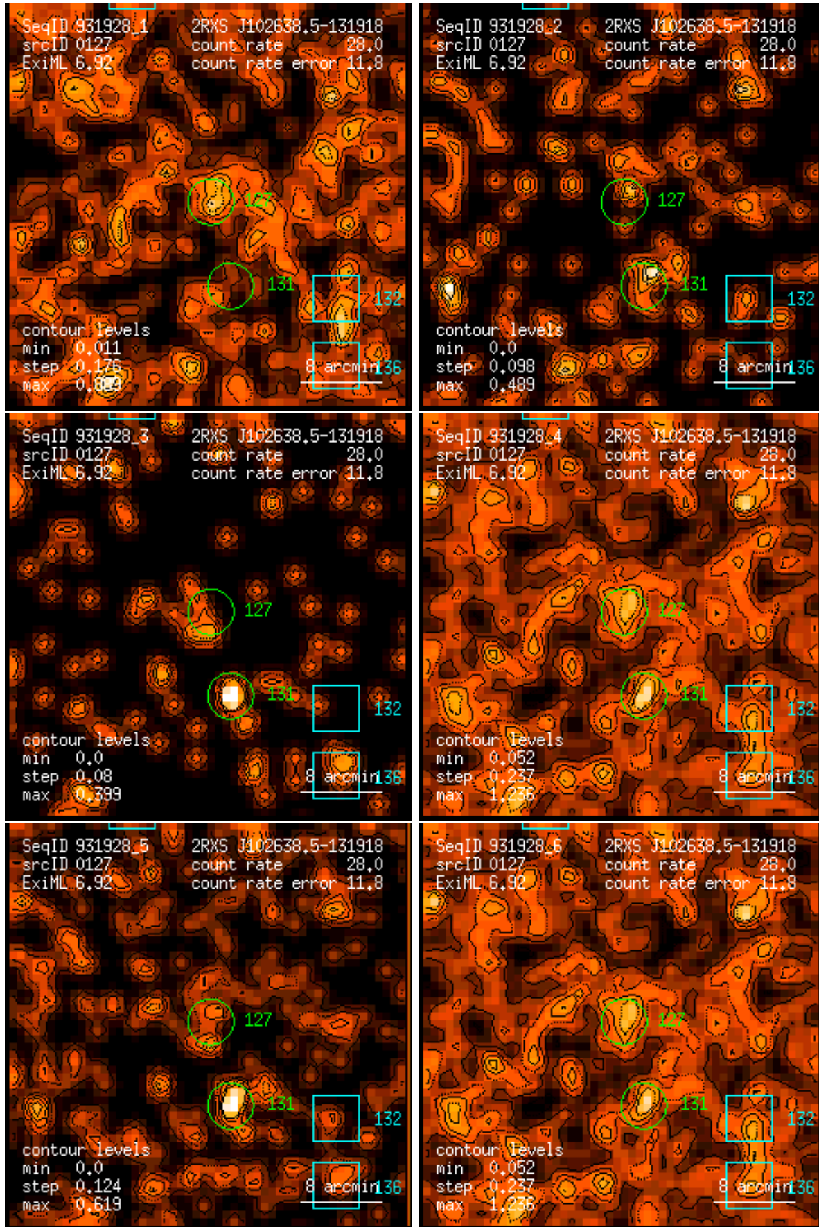
Figure 127: RASS 931928: detection 0127: band rate images, Gaussian filter: (1) PSPC channels 11 – 41, (2) 52 – 90, (3) 91 – 201, (4) 11 – 235, (5) 52 – 201, (6) 11 – 201. Broad band rates in counts/ks. Band rate contour levels in counts/ks/arcmin 2 .
