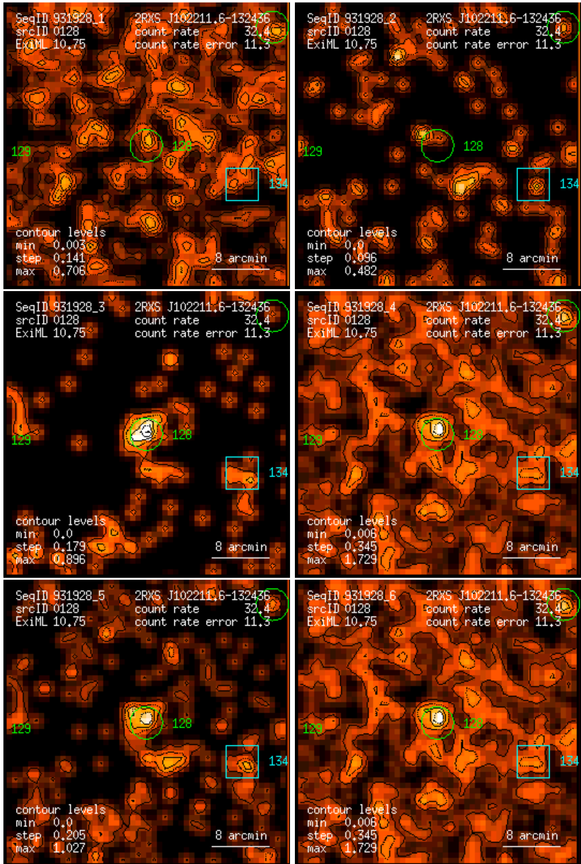
Figure 128: RASS 931928: detection 0128: band rate images, Gaussian filter: (1) PSPC channels 11 – 41, (2) 52 – 90, (3) 91 – 201, (4) 11 – 235, (5) 52 – 201, (6) 11 – 201. Broad band rates in counts/ks. Band rate contour levels in counts/ks/arcmin 2 .
