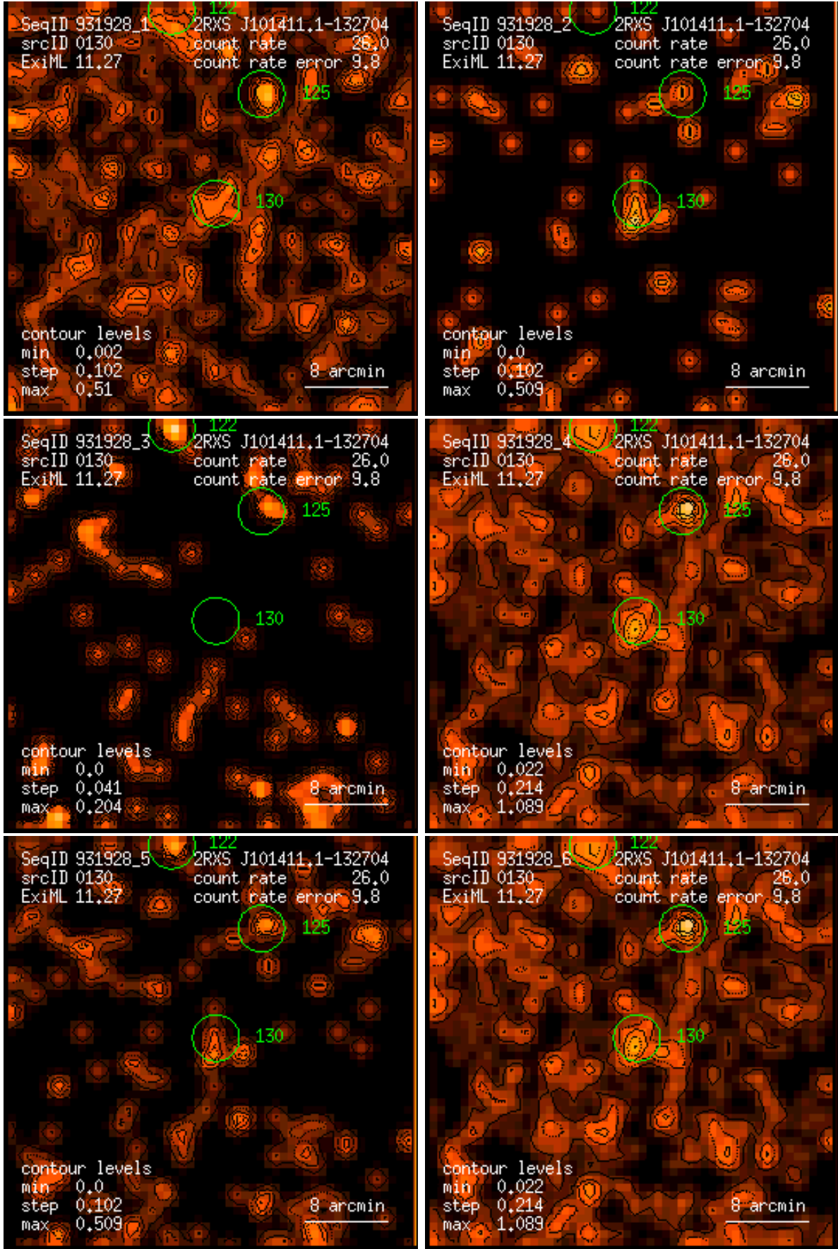
Figure 130: RASS 931928: detection 0130: band rate images, Gaussian filter: (1) PSPC channels 11 – 41, (2) 52 – 90, (3) 91 – 201, (4) 11 – 235, (5) 52 – 201, (6) 11 – 201. Broad band rates in counts/ks. Band rate contour levels in counts/ks/arcmin 2 .
