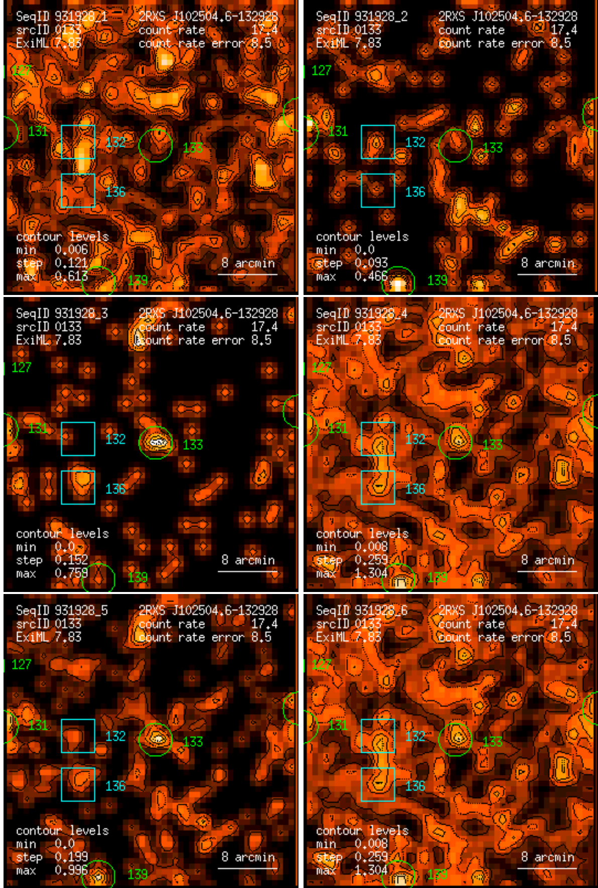
Figure 133: RASS 931928: detection 0133: band rate images, Gaussian filter: (1) PSPC channels 11 – 41, (2) 52 – 90, (3) 91 – 201, (4) 11 – 235, (5) 52 – 201, (6) 11 – 201. Broad band rates in counts/ks. Band rate contour levels in counts/ks/arcmin 2 .
