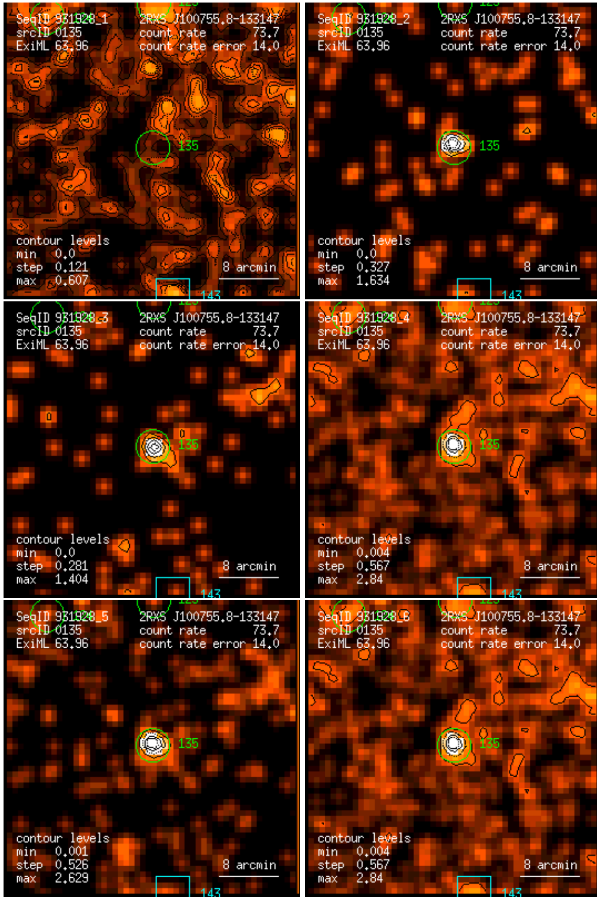
Figure 135: RASS 931928: detection 0135: band rate images, Gaussian filter: (1) PSPC channels 11 – 41, (2) 52 – 90, (3) 91 – 201, (4) 11 – 235, (5) 52 – 201, (6) 11 – 201. Broad band rates in counts/ks. Band rate contour levels in counts/ks/arcmin 2 .
