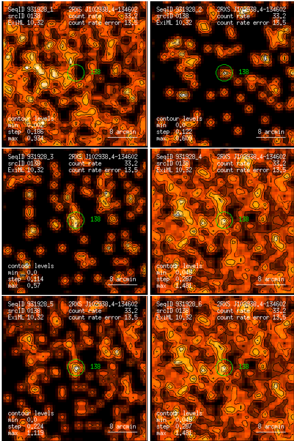
Figure 138: RASS 931928: detection 0138: band rate images, Gaussian filter: (1) PSPC channels 11 – 41, (2) 52 – 90, (3) 91 – 201, (4) 11 – 235, (5) 52 – 201, (6) 11 – 201. Broad band rates in counts/ks. Band rate contour levels in counts/ks/arcmin 2 .
