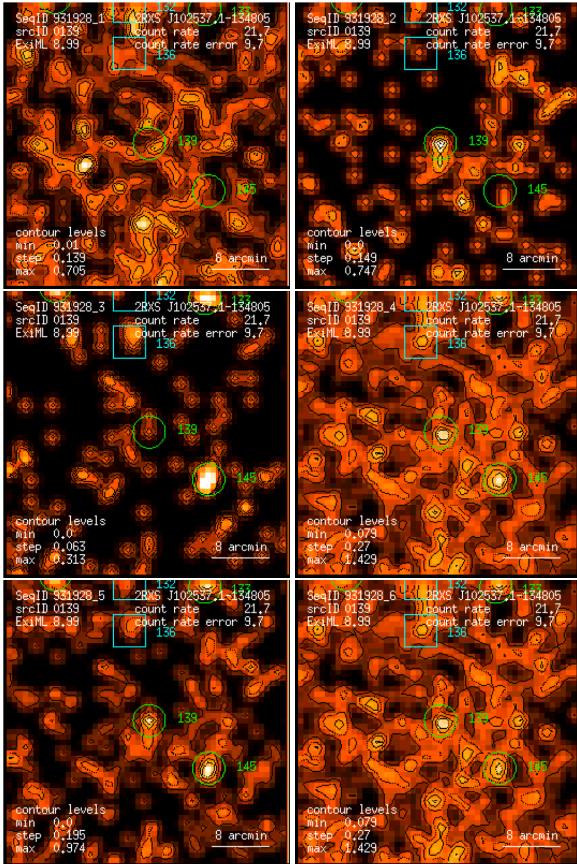
Figure 139: RASS 931928: detection 0139: band rate images, Gaussian filter: (1) PSPC channels 11 – 41, (2) 52 – 90, (3) 91 – 201, (4) 11 – 235, (5) 52 – 201, (6) 11 – 201. Broad band rates in counts/ks. Band rate contour levels in counts/ks/arcmin 2 .
