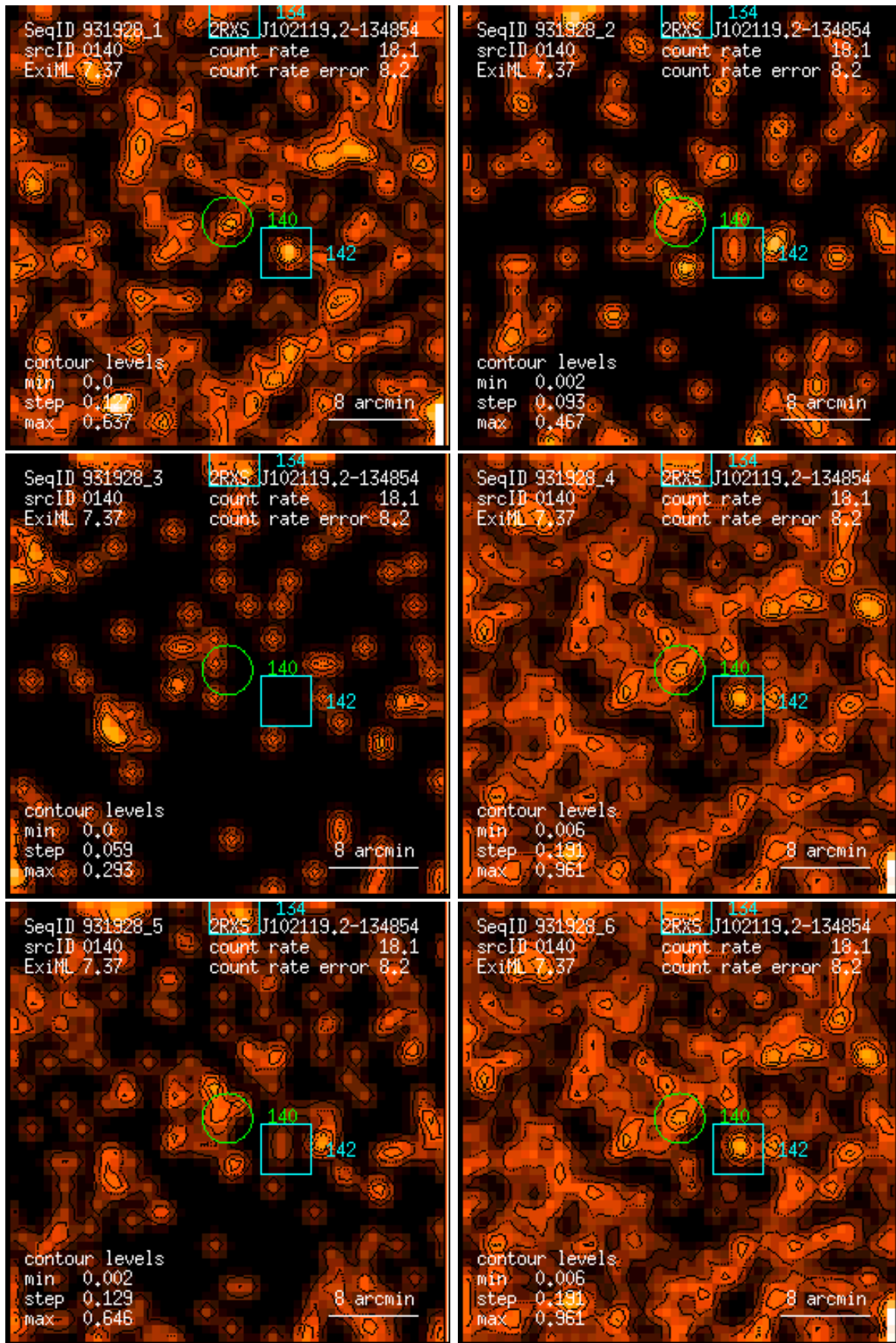
Figure 140: RASS 931928: detection 0140: band rate images, Gaussian filter: (1) PSPC channels 11 – 41, (2) 52 – 90, (3) 91 – 201, (4) 11 – 235, (5) 52 – 201, (6) 11 – 201. Broad band rates in counts/ks. Band rate contour levels in counts/ks/arcmin 2 .
