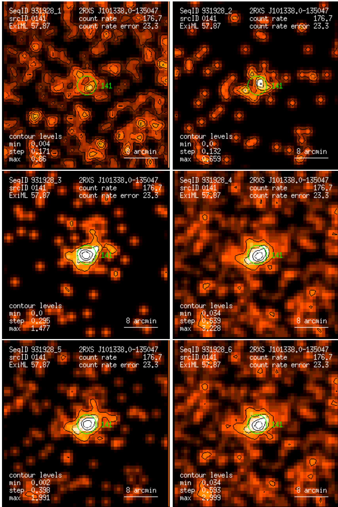
Figure 141: RASS 931928: detection 0141: band rate images, Gaussian filter: (1) PSPC channels 11 – 41, (2) 52 – 90, (3) 91 – 201, (4) 11 – 235, (5) 52 – 201, (6) 11 – 201. Broad band rates in counts/ks. Band rate contour levels in counts/ks/arcmin 2 .
