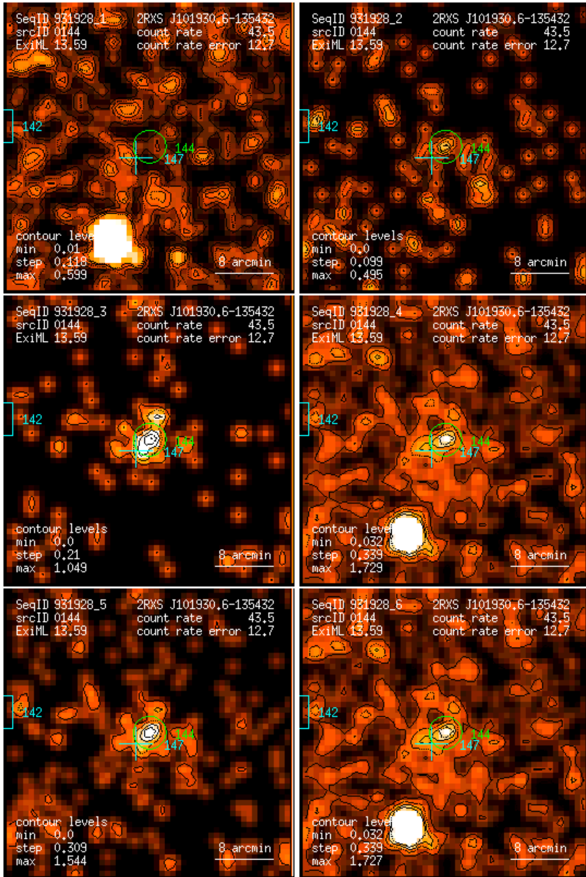
Figure 144: RASS 931928: detection 0144: band rate images, Gaussian filter: (1) PSPC channels 11 – 41, (2) 52 – 90, (3) 91 – 201, (4) 11 – 235, (5) 52 – 201, (6) 11 – 201. Broad band rates in counts/ks. Band rate contour levels in counts/ks/arcmin 2 .
