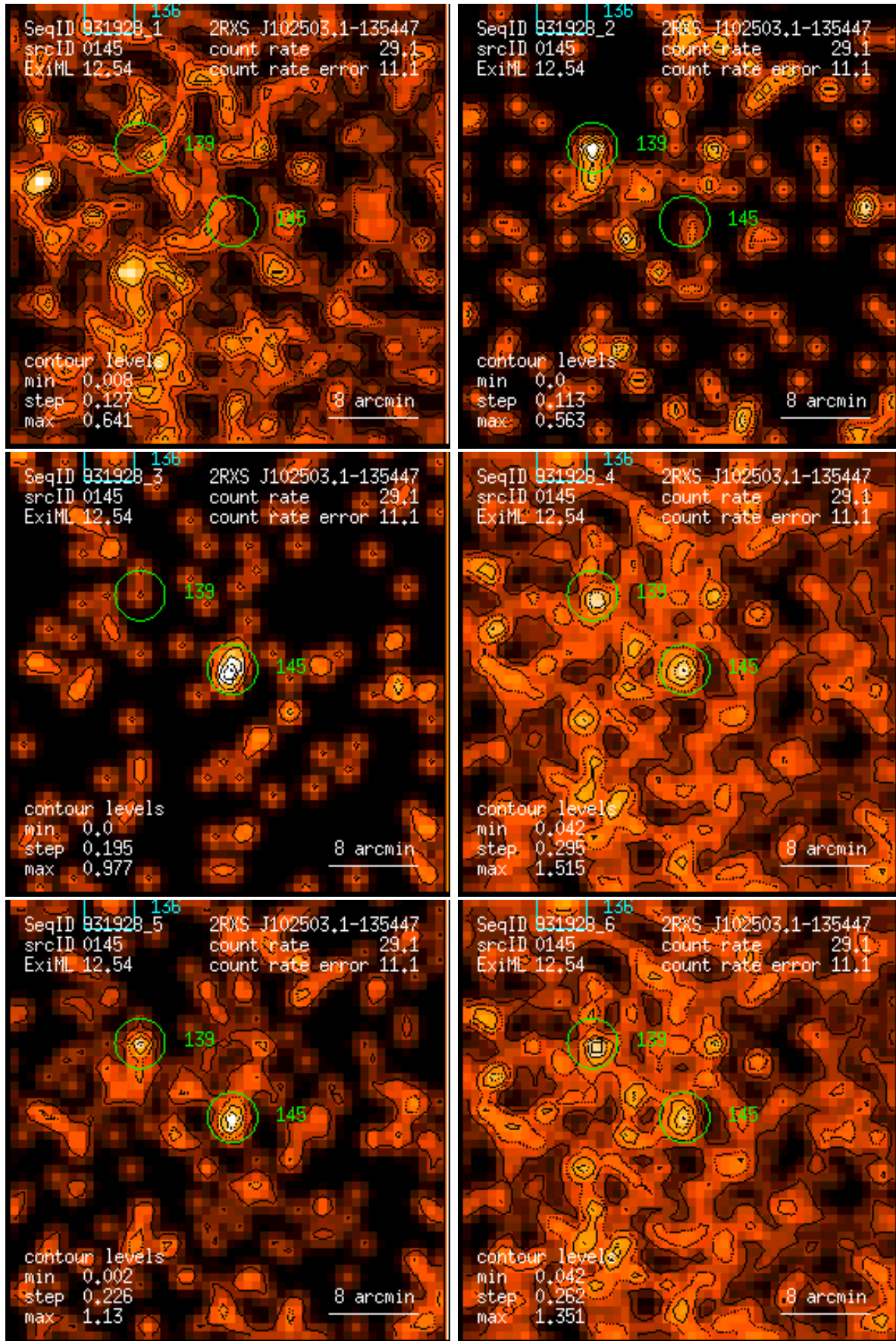
Figure 145: RASS 931928: detection 0145: band rate images, Gaussian filter: (1) PSPC channels 11 – 41, (2) 52 – 90, (3) 91 – 201, (4) 11 – 235, (5) 52 – 201, (6) 11 – 201. Broad band rates in counts/ks. Band rate contour levels in counts/ks/arcmin 2 .
