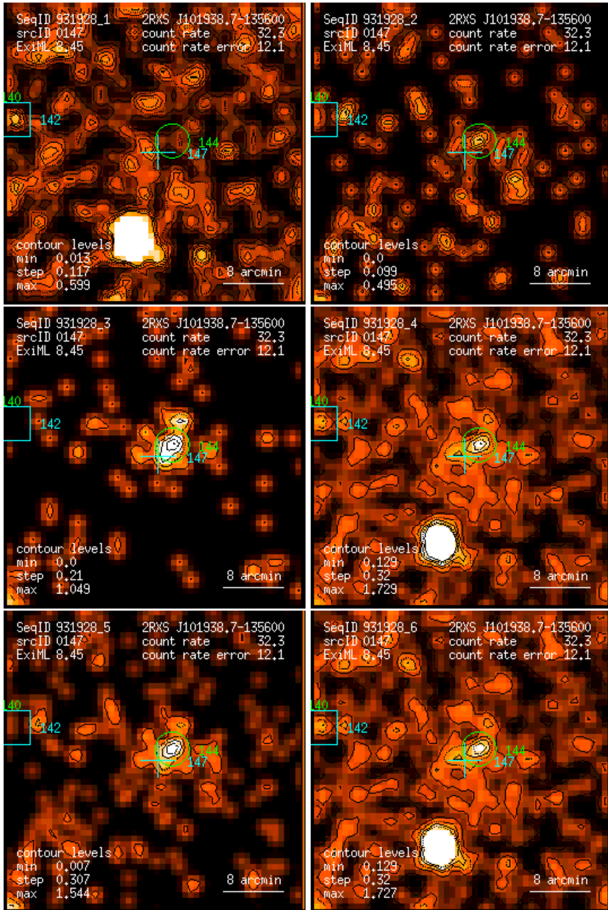
Figure 147: RASS 931928: detection 0147: band rate images, Gaussian filter: (1) PSPC channels 11 – 41, (2) 52 – 90, (3) 91 – 201, (4) 11 – 235, (5) 52 – 201, (6) 11 – 201. Broad band rates in counts/ks. Band rate contour levels in counts/ks/arcmin 2 .
